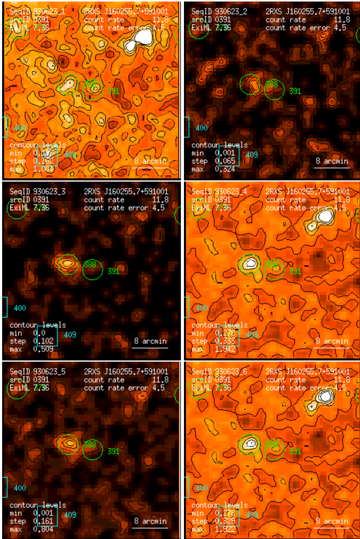
Figure 391: RASS 930623: detection 0391: band rate images, Gaussian filter: (1) PSPC channels 11 – 41, (2) 52 – 90, (3) 91 – 201, (4) 11 – 235, (5) 52 – 201, (6) 11 – 201. Broad band rates in counts/ks. Band rate contour levels in counts/ks/arcmin 2 .
