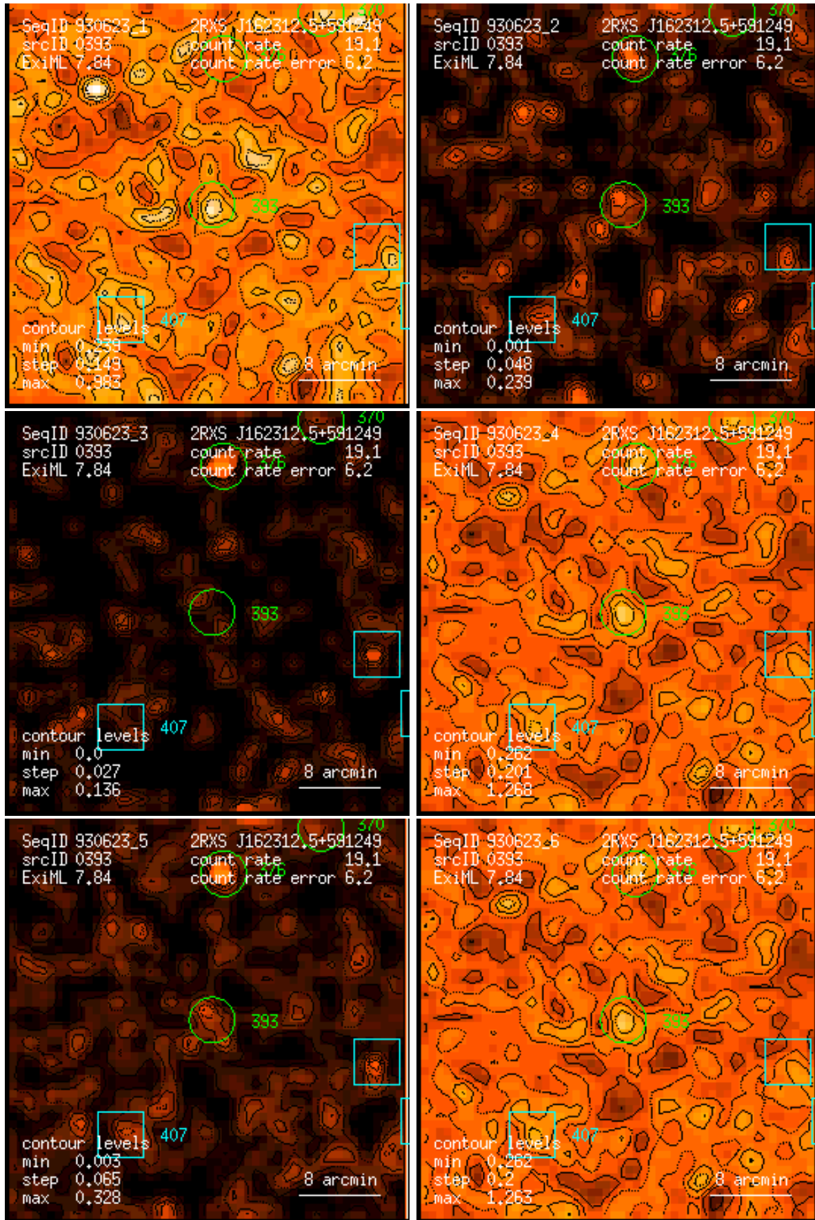
Figure 393: RASS 930623: detection 0393: band rate images, Gaussian filter: (1) PSPC channels 11 – 41, (2) 52 – 90, (3) 91 – 201, (4) 11 – 235, (5) 52 – 201, (6) 11 – 201. Broad band rates in counts/ks. Band rate contour levels in counts/ks/arcmin 2 .
