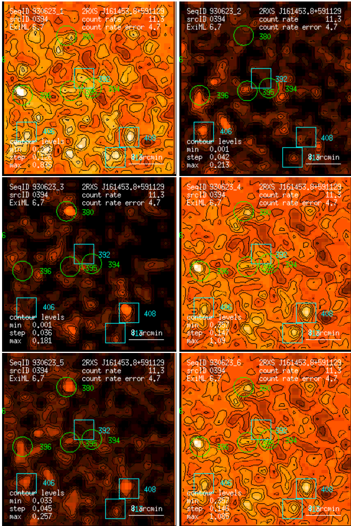
Figure 394: RASS 930623: detection 0394: band rate images, Gaussian filter: (1) PSPC channels 11 – 41, (2) 52 – 90, (3) 91 – 201, (4) 11 – 235, (5) 52 – 201, (6) 11 – 201. Broad band rates in counts/ks. Band rate contour levels in counts/ks/arcmin 2 .
