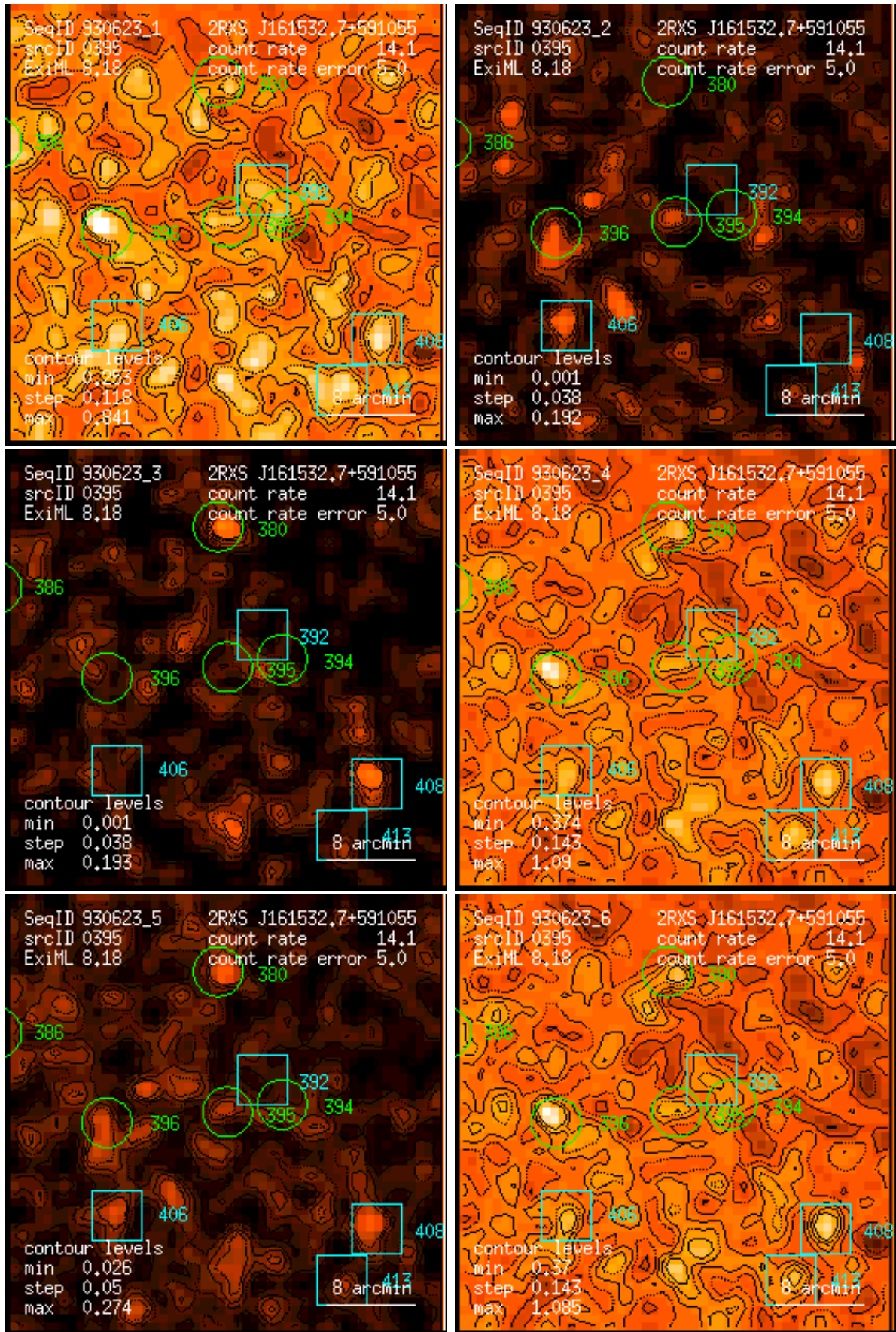
Figure 395: RASS 930623: detection 0395: band rate images, Gaussian filter: (1) PSPC channels 11 – 41, (2) 52 – 90, (3) 91 – 201, (4) 11 – 235, (5) 52 – 201, (6) 11 – 201. Broad band rates in counts/ks. Band rate contour levels in counts/ks/arcmin 2 .
