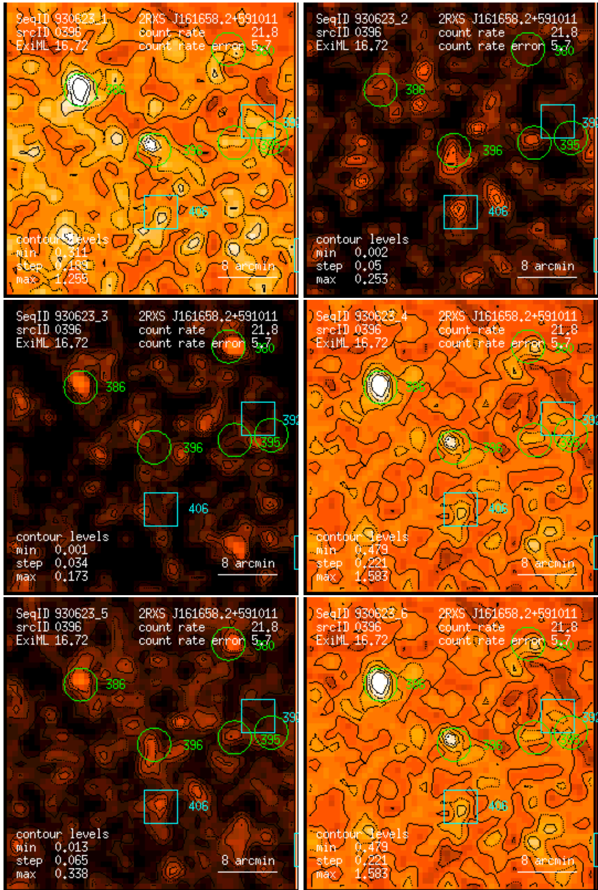
Figure 396: RASS 930623: detection 0396: band rate images, Gaussian filter: (1) PSPC channels 11 – 41, (2) 52 – 90, (3) 91 – 201, (4) 11 – 235, (5) 52 – 201, (6) 11 – 201. Broad band rates in counts/ks. Band rate contour levels in counts/ks/arcmin 2 .
