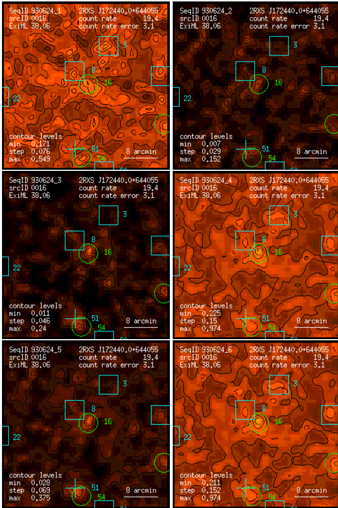
Figure 16: RASS 930624: detection 0016: band rate images, Gaussian filter: (1) PSPC channels 11 – 41, (2) 52 – 90, (3) 91 – 201, (4) 11 – 235, (5) 52 – 201, (6) 11 – 201. Broad band rates in counts/ks. Band rate contour levels in counts/ks/arcmin 2 .
