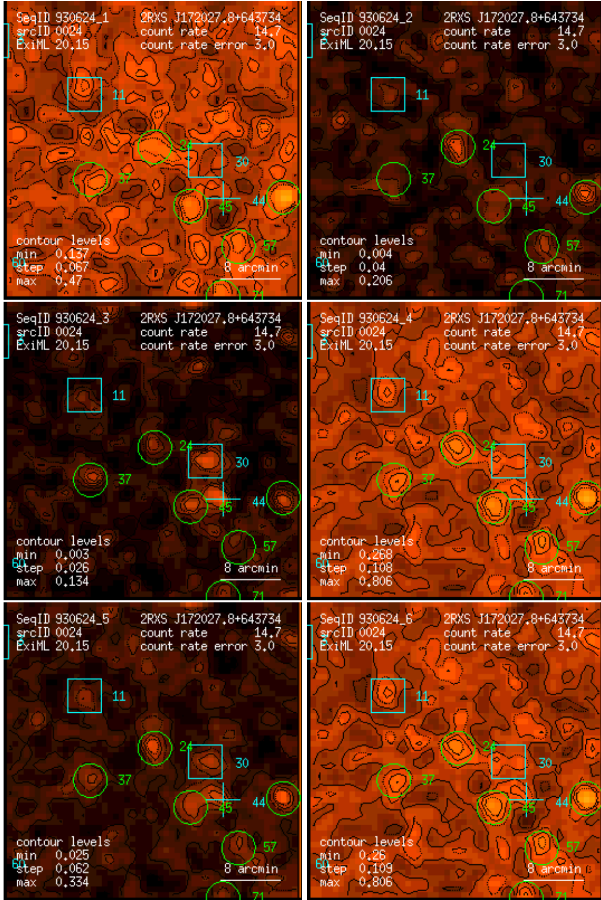
Figure 24: RASS 930624: detection 0024: band rate images, Gaussian filter: (1) PSPC channels 11 – 41, (2) 52 – 90, (3) 91 – 201, (4) 11 – 235, (5) 52 – 201, (6) 11 – 201. Broad band rates in counts/ks. Band rate contour levels in counts/ks/arcmin 2 .
