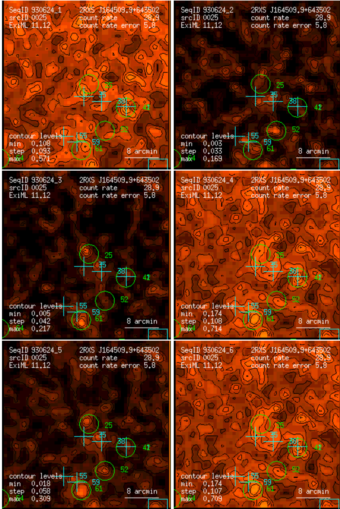
Figure 25: RASS 930624: detection 0025: band rate images, Gaussian filter: (1) PSPC channels 11 – 41, (2) 52 – 90, (3) 91 – 201, (4) 11 – 235, (5) 52 – 201, (6) 11 – 201. Broad band rates in counts/ks. Band rate contour levels in counts/ks/arcmin 2 .
