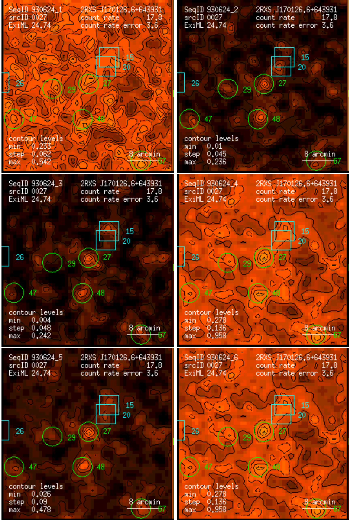
Figure 27: RASS 930624: detection 0027: band rate images, Gaussian filter: (1) PSPC channels 11 – 41, (2) 52 – 90, (3) 91 – 201, (4) 11 – 235, (5) 52 – 201, (6) 11 – 201. Broad band rates in counts/ks. Band rate contour levels in counts/ks/arcmin 2 .
