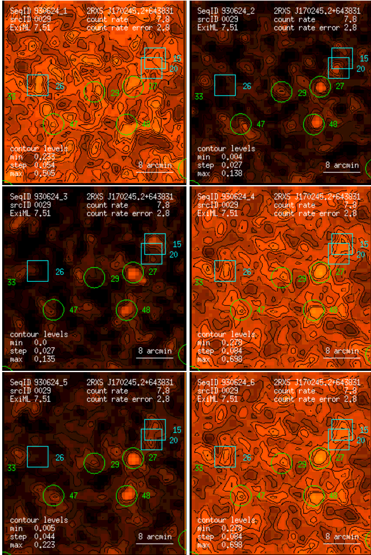
Figure 29: RASS 930624: detection 0029: band rate images, Gaussian filter: (1) PSPC channels 11 – 41, (2) 52 – 90, (3) 91 – 201, (4) 11 – 235, (5) 52 – 201, (6) 11 – 201. Broad band rates in counts/ks. Band rate contour levels in counts/ks/arcmin 2 .
