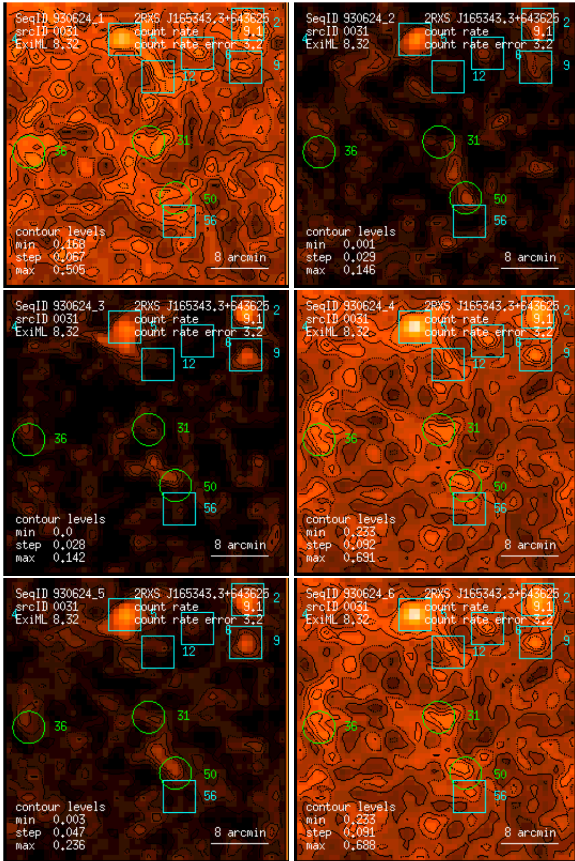
Figure 31: RASS 930624: detection 0031: band rate images, Gaussian filter: (1) PSPC channels 11 – 41, (2) 52 – 90, (3) 91 – 201, (4) 11 – 235, (5) 52 – 201, (6) 11 – 201. Broad band rates in counts/ks. Band rate contour levels in counts/ks/arcmin 2 .
