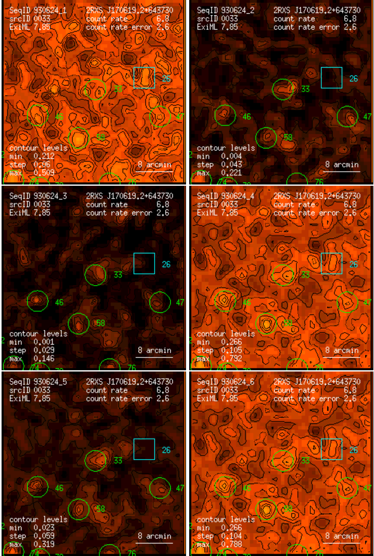
Figure 33: RASS 930624: detection 0033: band rate images, Gaussian filter: (1) PSPC channels 11 – 41, (2) 52 – 90, (3) 91 – 201, (4) 11 – 235, (5) 52 – 201, (6) 11 – 201. Broad band rates in counts/ks. Band rate contour levels in counts/ks/arcmin 2 .
