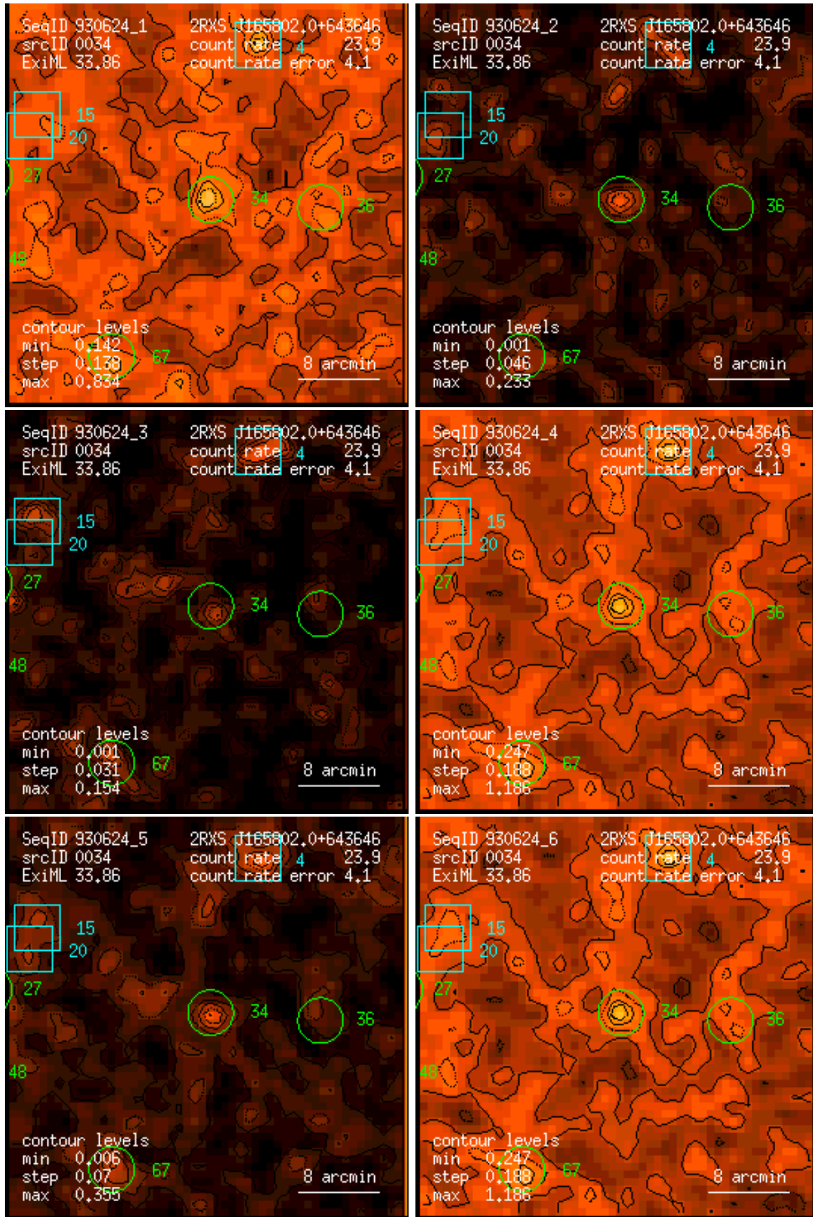
Figure 34: RASS 930624: detection 0034: band rate images, Gaussian filter: (1) PSPC channels 11 – 41, (2) 52 – 90, (3) 91 – 201, (4) 11 – 235, (5) 52 – 201, (6) 11 – 201. Broad band rates in counts/ks. Band rate contour levels in counts/ks/arcmin 2 .
