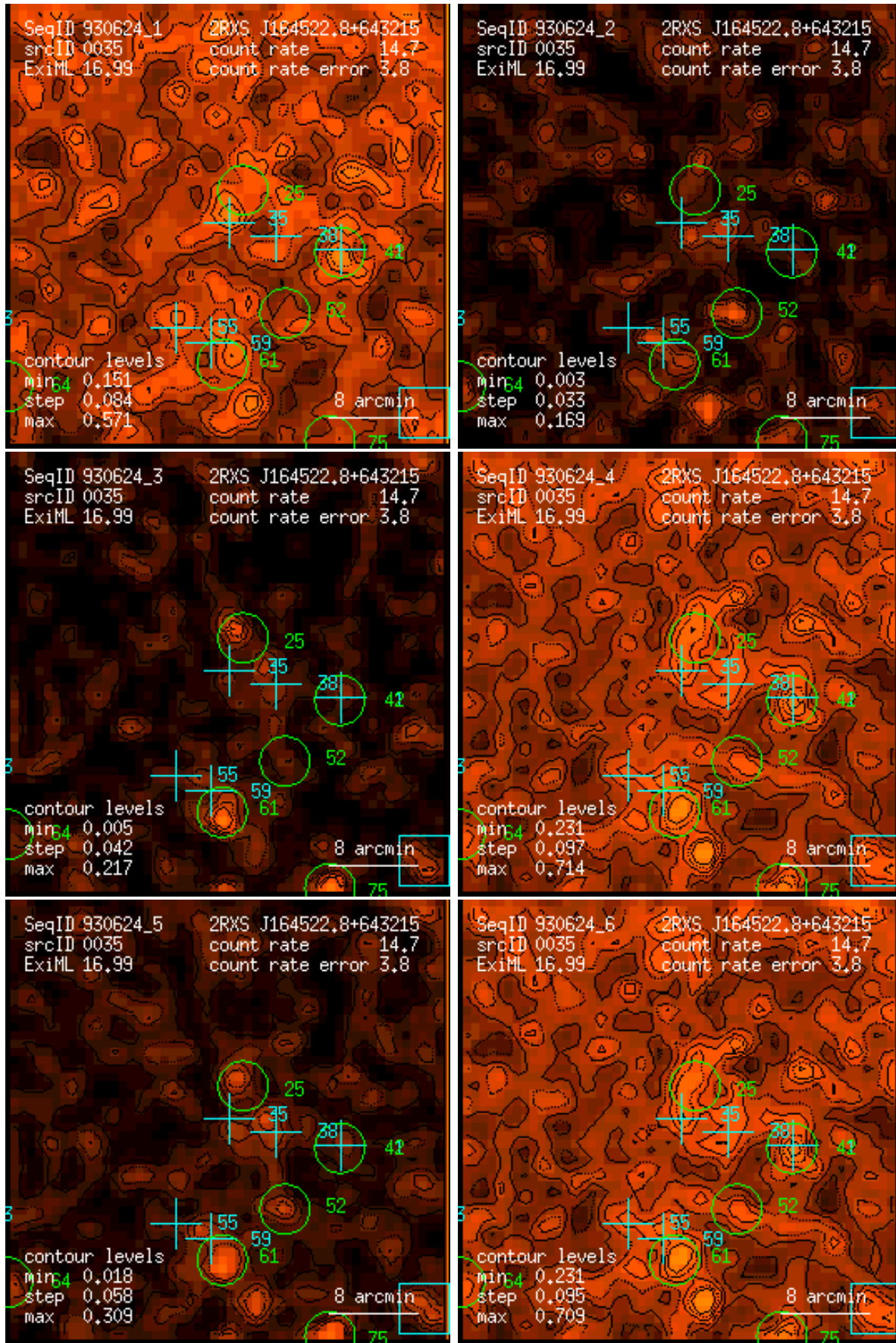
Figure 35: RASS 930624: detection 0035: band rate images, Gaussian filter: (1) PSPC channels 11 – 41, (2) 52 – 90, (3) 91 – 201, (4) 11 – 235, (5) 52 – 201, (6) 11 – 201. Broad band rates in counts/ks. Band rate contour levels in counts/ks/arcmin 2 .
