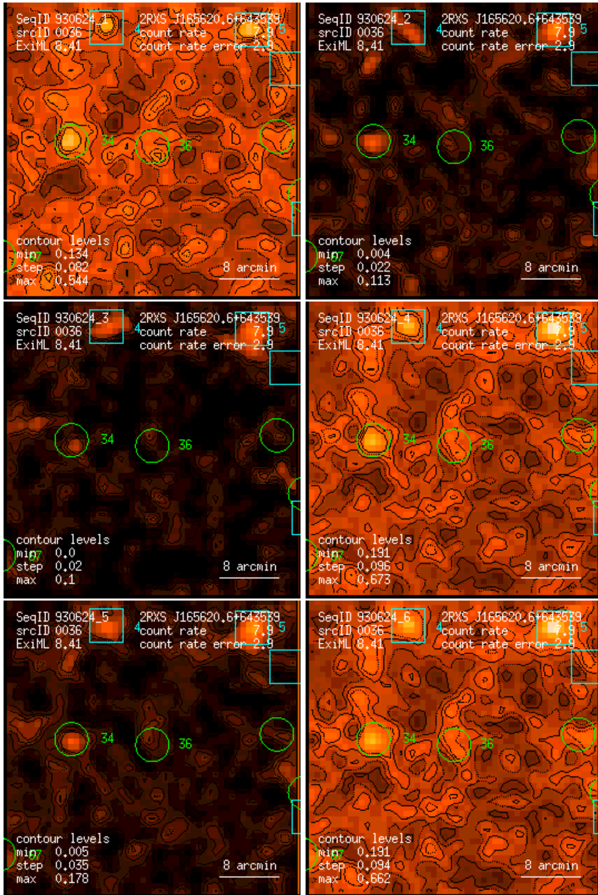
Figure 36: RASS 930624: detection 0036: band rate images, Gaussian filter: (1) PSPC channels 11 – 41, (2) 52 – 90, (3) 91 – 201, (4) 11 – 235, (5) 52 – 201, (6) 11 – 201. Broad band rates in counts/ks. Band rate contour levels in counts/ks/arcmin 2 .
