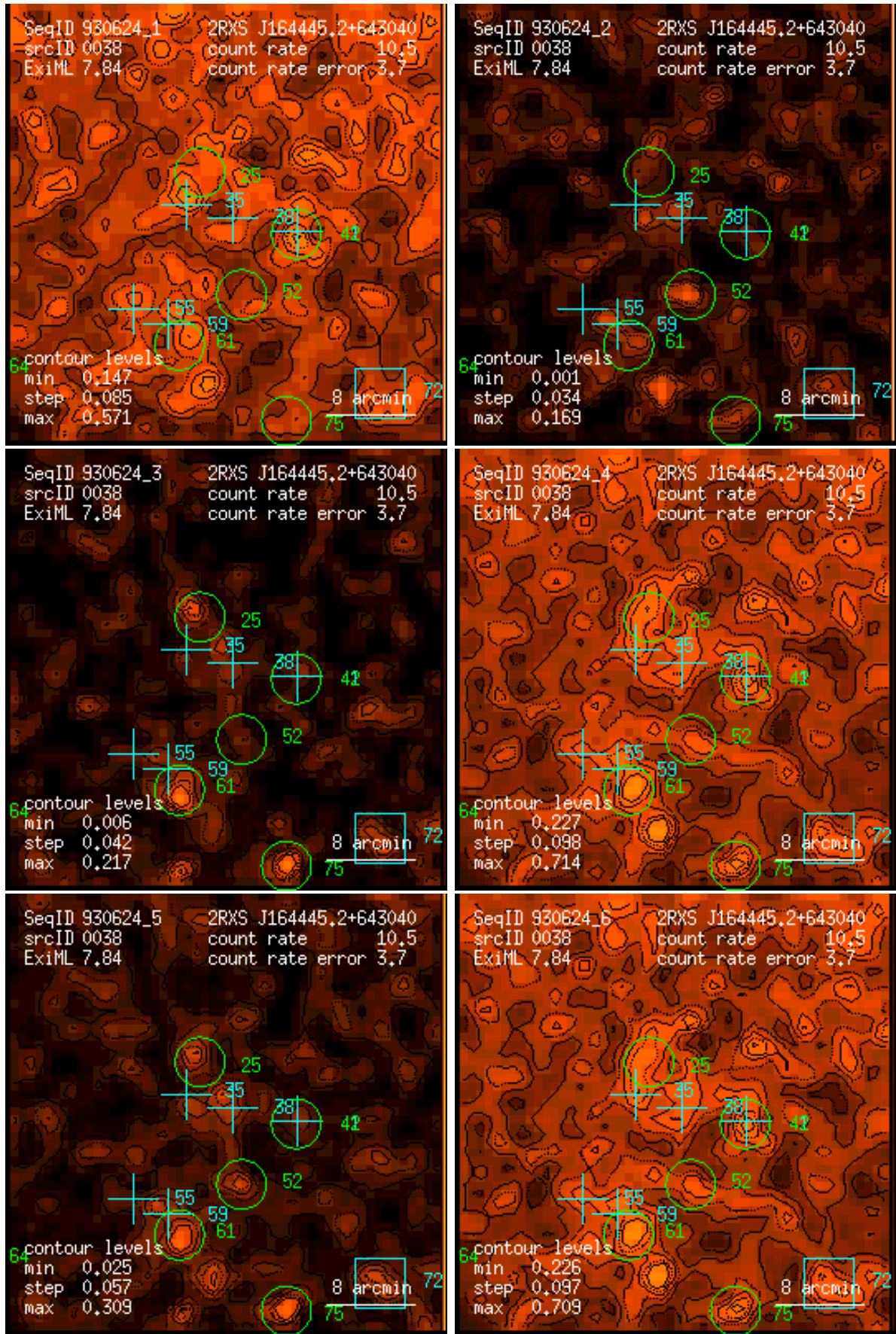
Figure 38: RASS 930624: detection 0038: band rate images, Gaussian filter: (1) PSPC channels 11 – 41, (2) 52 – 90, (3) 91 – 201, (4) 11 – 235, (5) 52 – 201, (6) 11 – 201. Broad band rates in counts/ks. Band rate contour levels in counts/ks/arcmin 2 .
