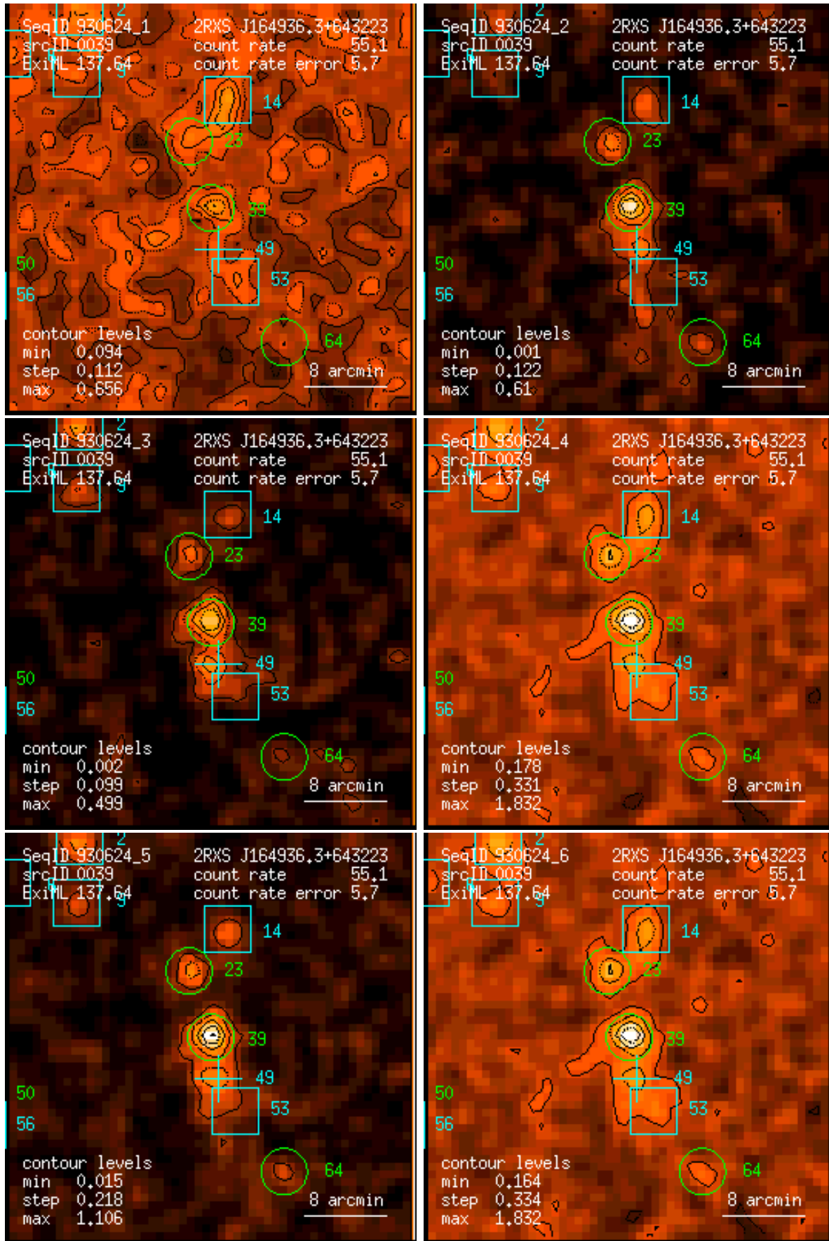
Figure 39: RASS 930624: detection 0039: band rate images, Gaussian filter: (1) PSPC channels 11 – 41, (2) 52 – 90, (3) 91 – 201, (4) 11 – 235, (5) 52 – 201, (6) 11 – 201. Broad band rates in counts/ks. Band rate contour levels in counts/ks/arcmin 2 .
