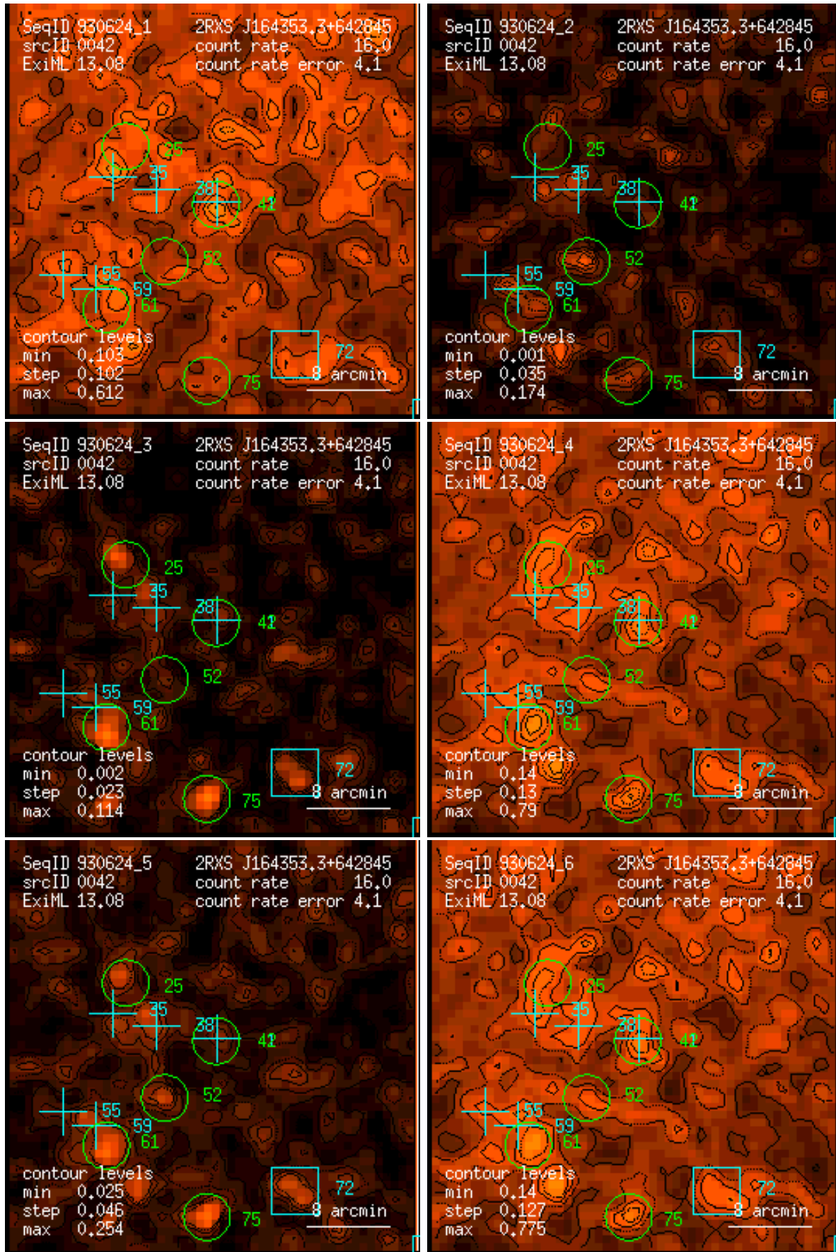
Figure 42: RASS 930624: detection 0042: band rate images, Gaussian filter: (1) PSPC channels 11 – 41, (2) 52 – 90, (3) 91 – 201, (4) 11 – 235, (5) 52 – 201, (6) 11 – 201. Broad band rates in counts/ks. Band rate contour levels in counts/ks/arcmin 2 .
