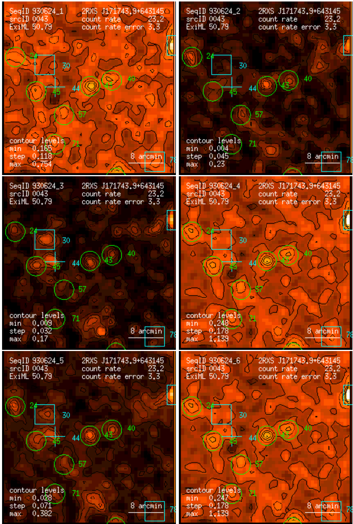
Figure 43: RASS 930624: detection 0043: band rate images, Gaussian filter: (1) PSPC channels 11 – 41, (2) 52 – 90, (3) 91 – 201, (4) 11 – 235, (5) 52 – 201, (6) 11 – 201. Broad band rates in counts/ks. Band rate contour levels in counts/ks/arcmin 2 .
