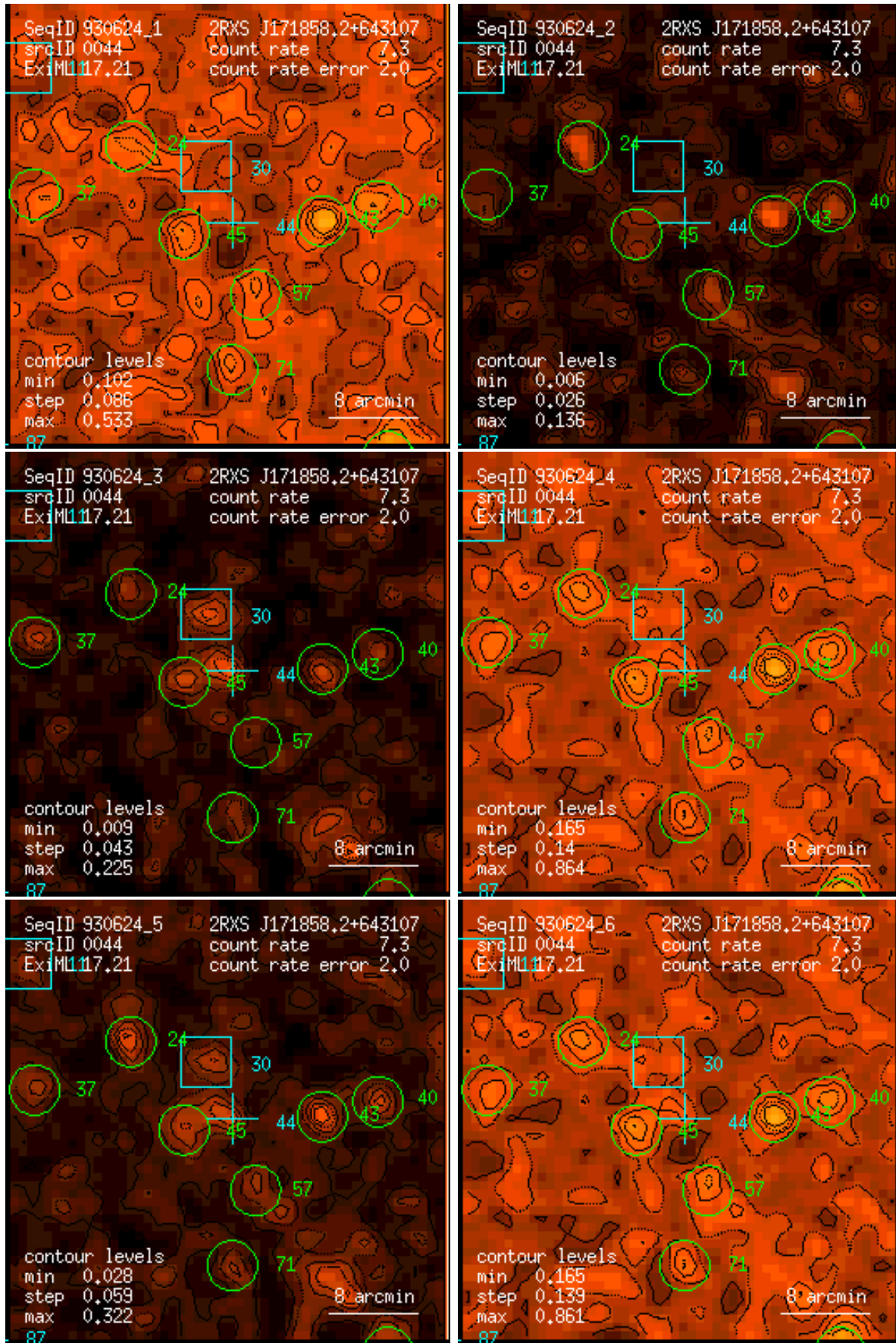
Figure 44: RASS 930624: detection 0044: band rate images, Gaussian filter: (1) PSPC channels 11 – 41, (2) 52 – 90, (3) 91 – 201, (4) 11 – 235, (5) 52 – 201, (6) 11 – 201. Broad band rates in counts/ks. Band rate contour levels in counts/ks/arcmin 2 .
