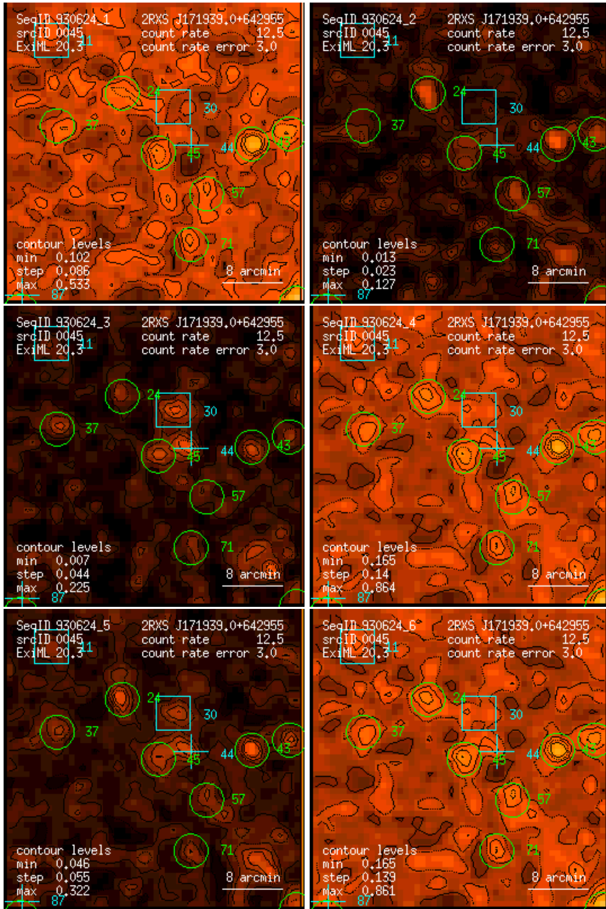
Figure 45: RASS 930624: detection 0045: band rate images, Gaussian filter: (1) PSPC channels 11 – 41, (2) 52 – 90, (3) 91 – 201, (4) 11 – 235, (5) 52 – 201, (6) 11 – 201. Broad band rates in counts/ks. Band rate contour levels in counts/ks/arcmin 2 .
