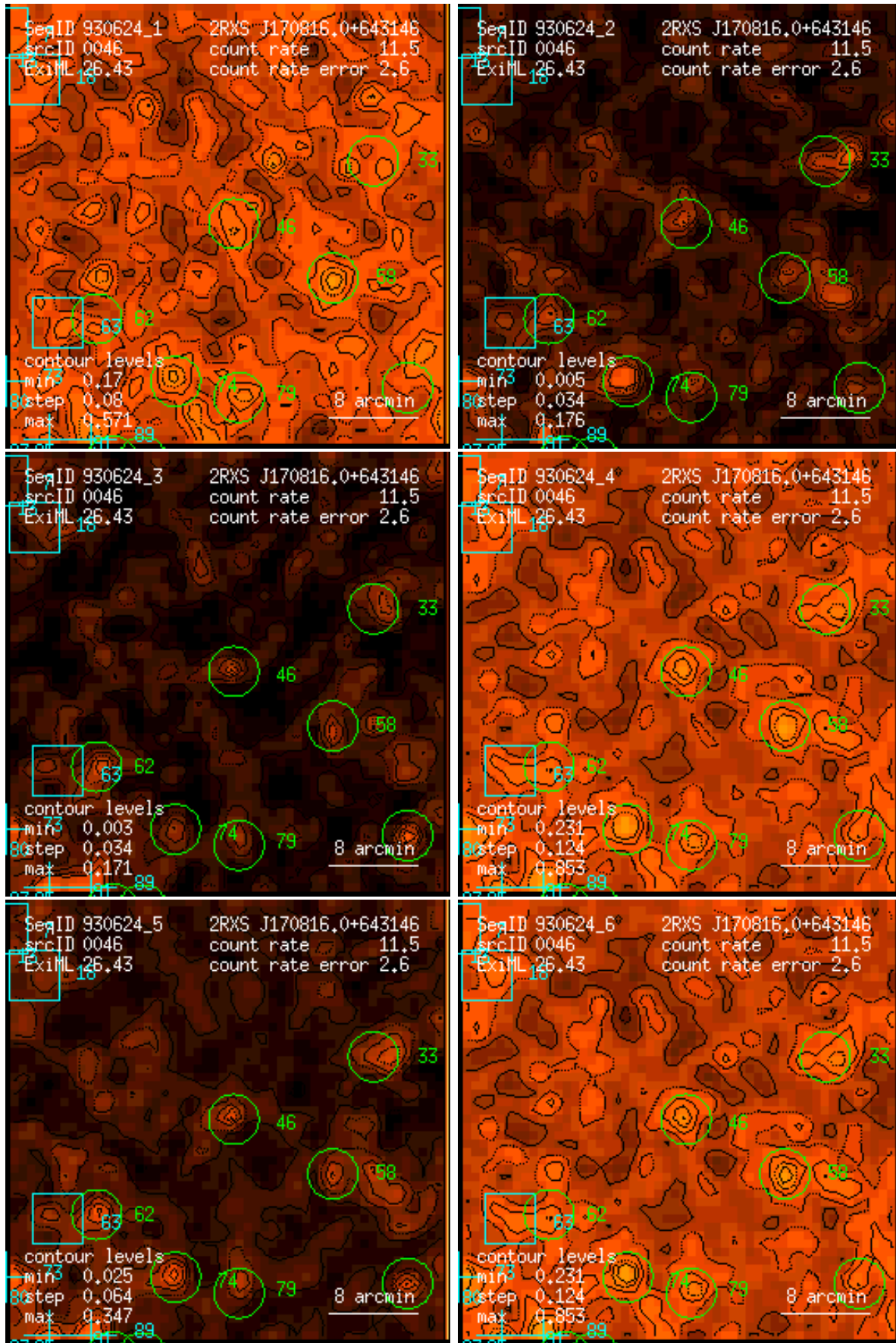
Figure 46: RASS 930624: detection 0046: band rate images, Gaussian filter: (1) PSPC channels 11 – 41, (2) 52 – 90, (3) 91 – 201, (4) 11 – 235, (5) 52 – 201, (6) 11 – 201. Broad band rates in counts/ks. Band rate contour levels in counts/ks/arcmin 2 .
