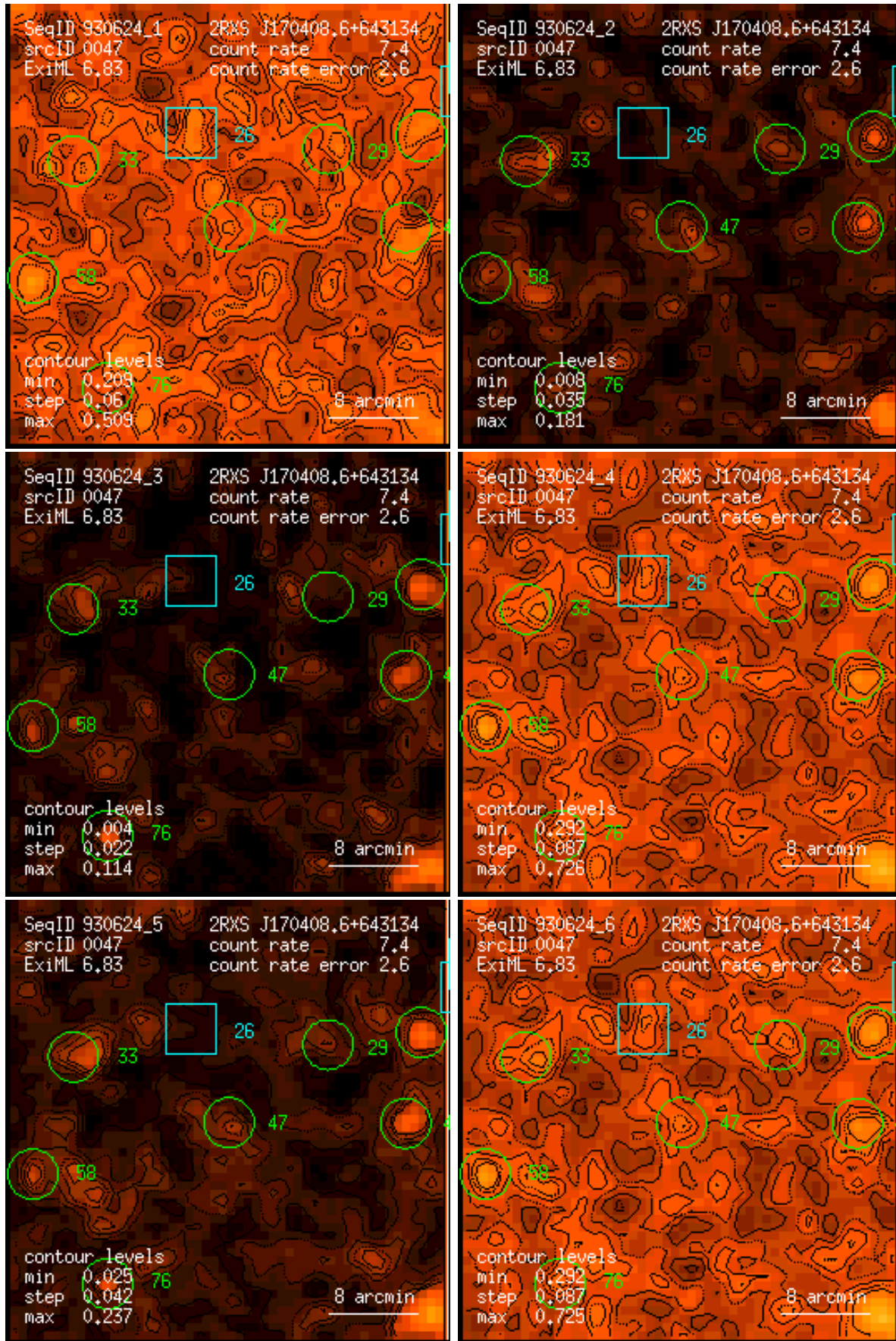
Figure 47: RASS 930624: detection 0047: band rate images, Gaussian filter: (1) PSPC channels 11 – 41, (2) 52 – 90, (3) 91 – 201, (4) 11 – 235, (5) 52 – 201, (6) 11 – 201. Broad band rates in counts/ks. Band rate contour levels in counts/ks/arcmin 2 .
