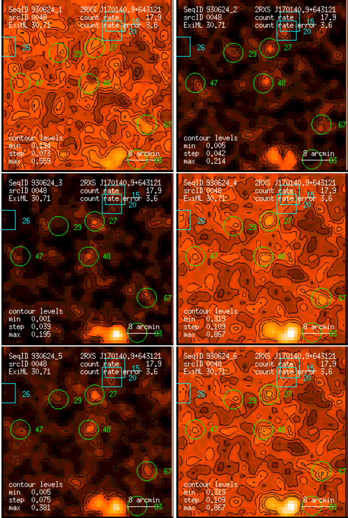
Figure 48: RASS 930624: detection 0048: band rate images, Gaussian filter: (1) PSPC channels 11 – 41, (2) 52 – 90, (3) 91 – 201, (4) 11 – 235, (5) 52 – 201, (6) 11 – 201. Broad band rates in counts/ks. Band rate contour levels in counts/ks/arcmin 2 .
