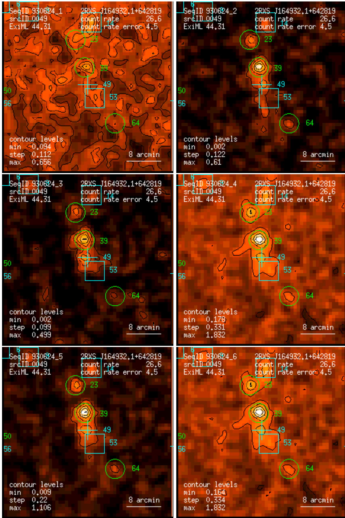
Figure 49: RASS 930624: detection 0049: band rate images, Gaussian filter: (1) PSPC channels 11 – 41, (2) 52 – 90, (3) 91 – 201, (4) 11 – 235, (5) 52 – 201, (6) 11 – 201. Broad band rates in counts/ks. Band rate contour levels in counts/ks/arcmin 2 .
