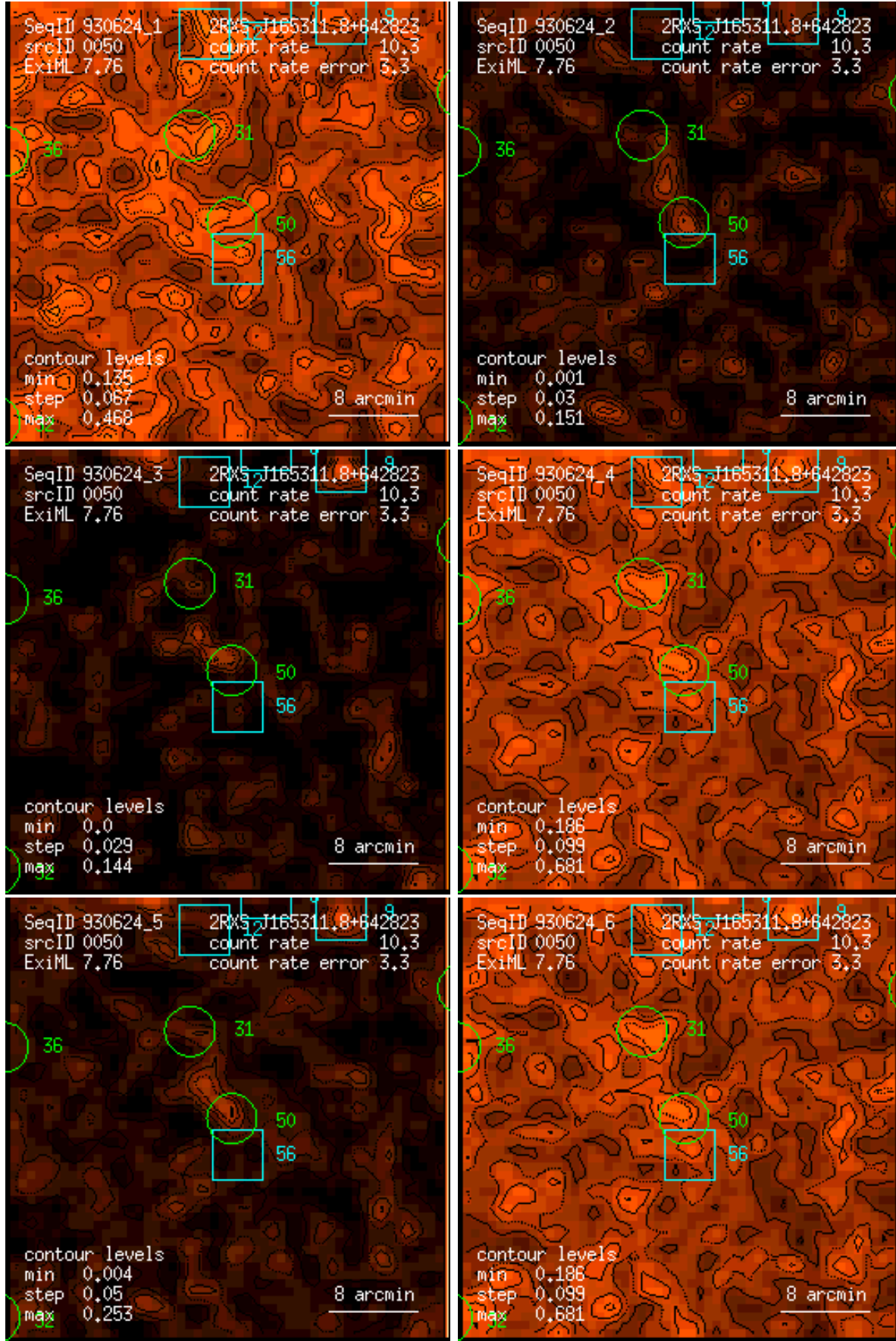
Figure 50: RASS 930624: detection 0050: band rate images, Gaussian filter: (1) PSPC channels 11 – 41, (2) 52 – 90, (3) 91 – 201, (4) 11 – 235, (5) 52 – 201, (6) 11 – 201. Broad band rates in counts/ks. Band rate contour levels in counts/ks/arcmin 2 .
