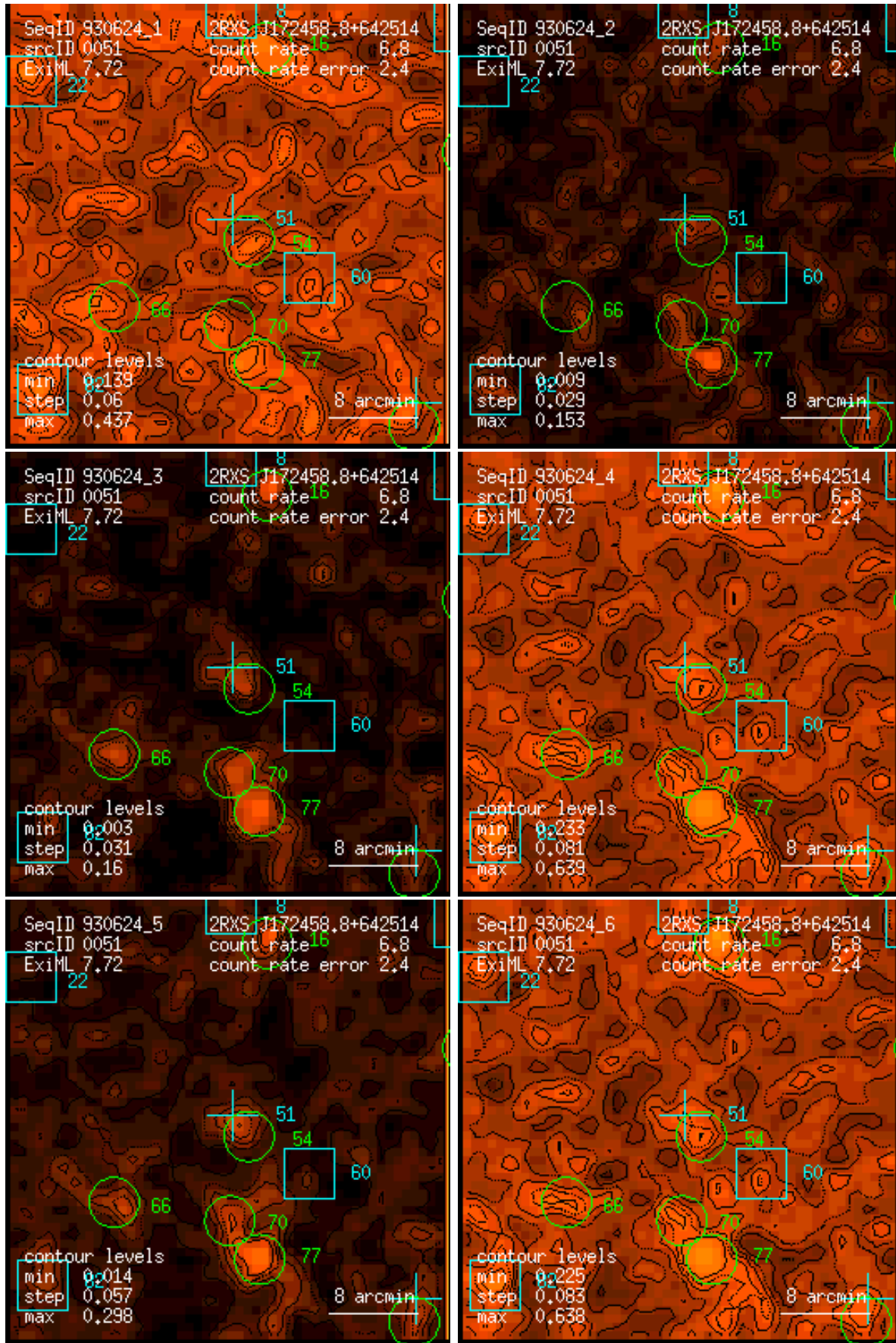
Figure 51: RASS 930624: detection 0051: band rate images, Gaussian filter: (1) PSPC channels 11 – 41, (2) 52 – 90, (3) 91 – 201, (4) 11 – 235, (5) 52 – 201, (6) 11 – 201. Broad band rates in counts/ks. Band rate contour levels in counts/ks/arcmin 2 .
