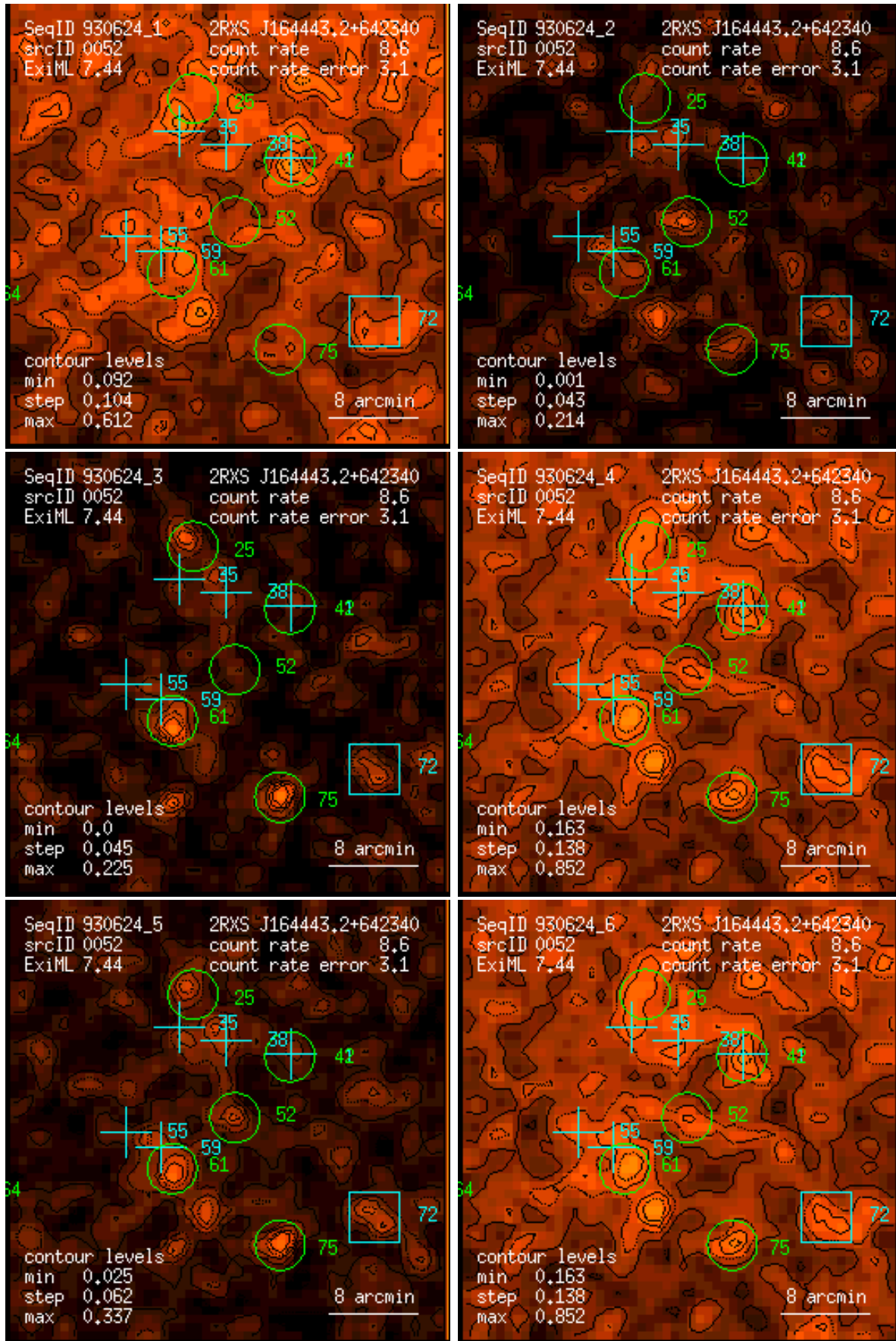
Figure 52: RASS 930624: detection 0052: band rate images, Gaussian filter: (1) PSPC channels 11 – 41, (2) 52 – 90, (3) 91 – 201, (4) 11 – 235, (5) 52 – 201, (6) 11 – 201. Broad band rates in counts/ks. Band rate contour levels in counts/ks/arcmin 2 .
