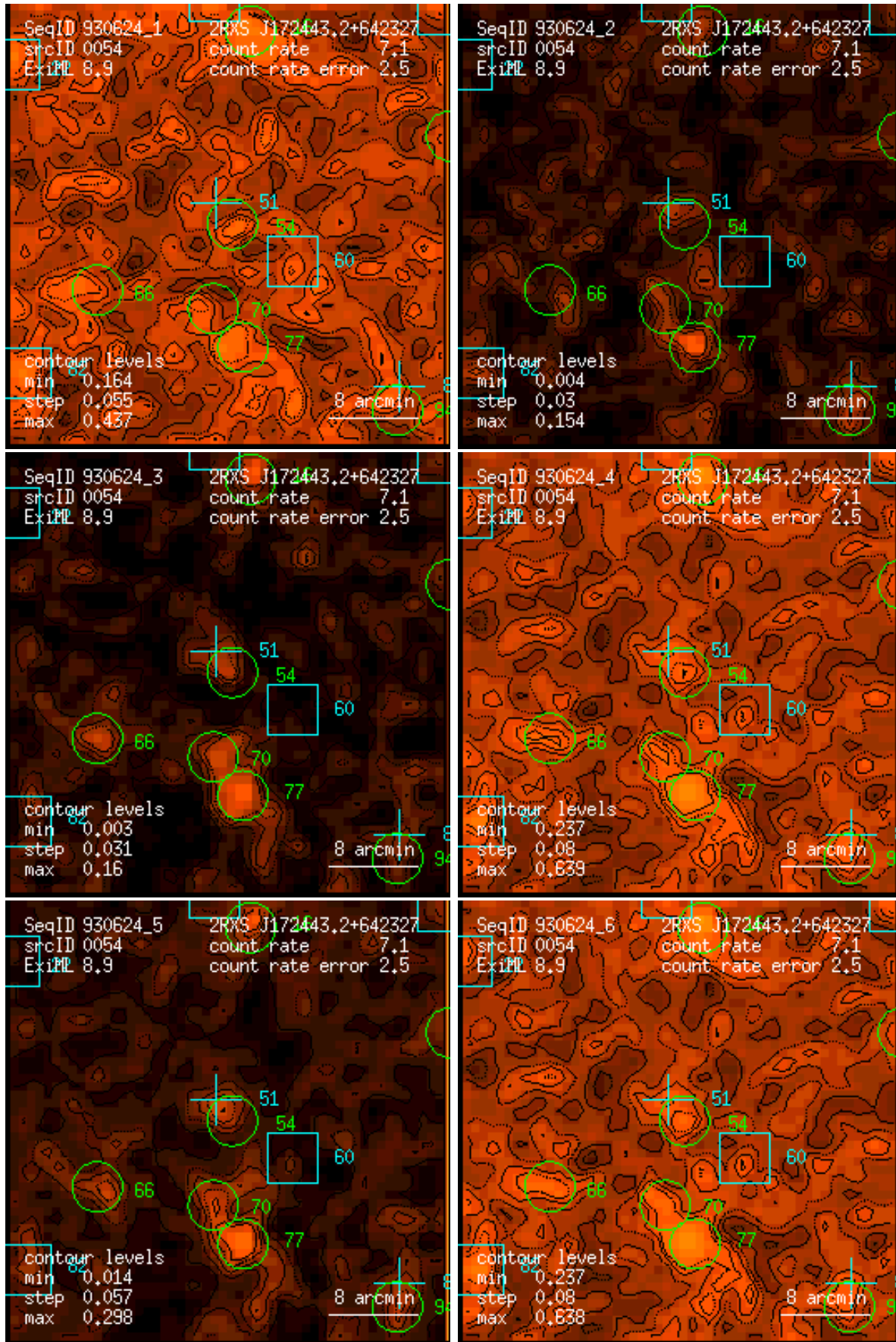
Figure 54: RASS 930624: detection 0054: band rate images, Gaussian filter: (1) PSPC channels 11 – 41, (2) 52 – 90, (3) 91 – 201, (4) 11 – 235, (5) 52 – 201, (6) 11 – 201. Broad band rates in counts/ks. Band rate contour levels in counts/ks/arcmin 2 .
