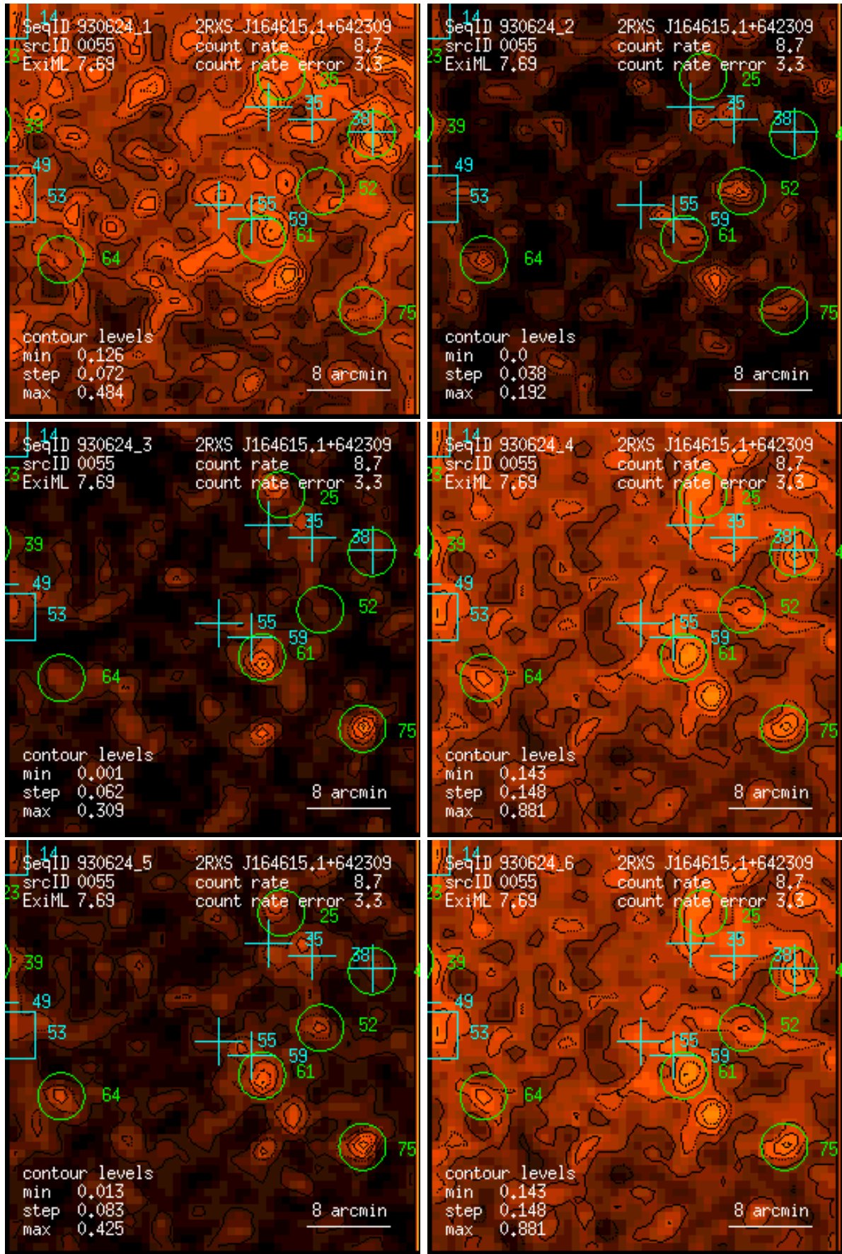
Figure 55: RASS 930624: detection 0055: band rate images, Gaussian filter: (1) PSPC channels 11 – 41, (2) 52 – 90, (3) 91 – 201, (4) 11 – 235, (5) 52 – 201, (6) 11 – 201. Broad band rates in counts/ks. Band rate contour levels in counts/ks/arcmin 2 .
