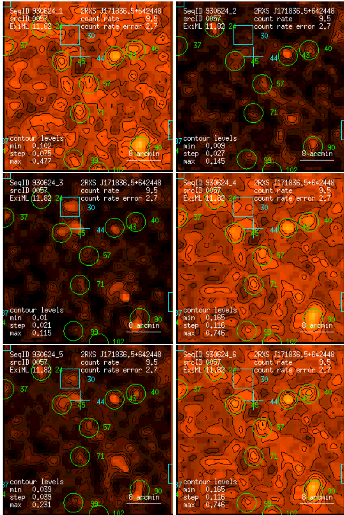
Figure 57: RASS 930624: detection 0057: band rate images, Gaussian filter: (1) PSPC channels 11 – 41, (2) 52 – 90, (3) 91 – 201, (4) 11 – 235, (5) 52 – 201, (6) 11 – 201. Broad band rates in counts/ks. Band rate contour levels in counts/ks/arcmin 2 .
