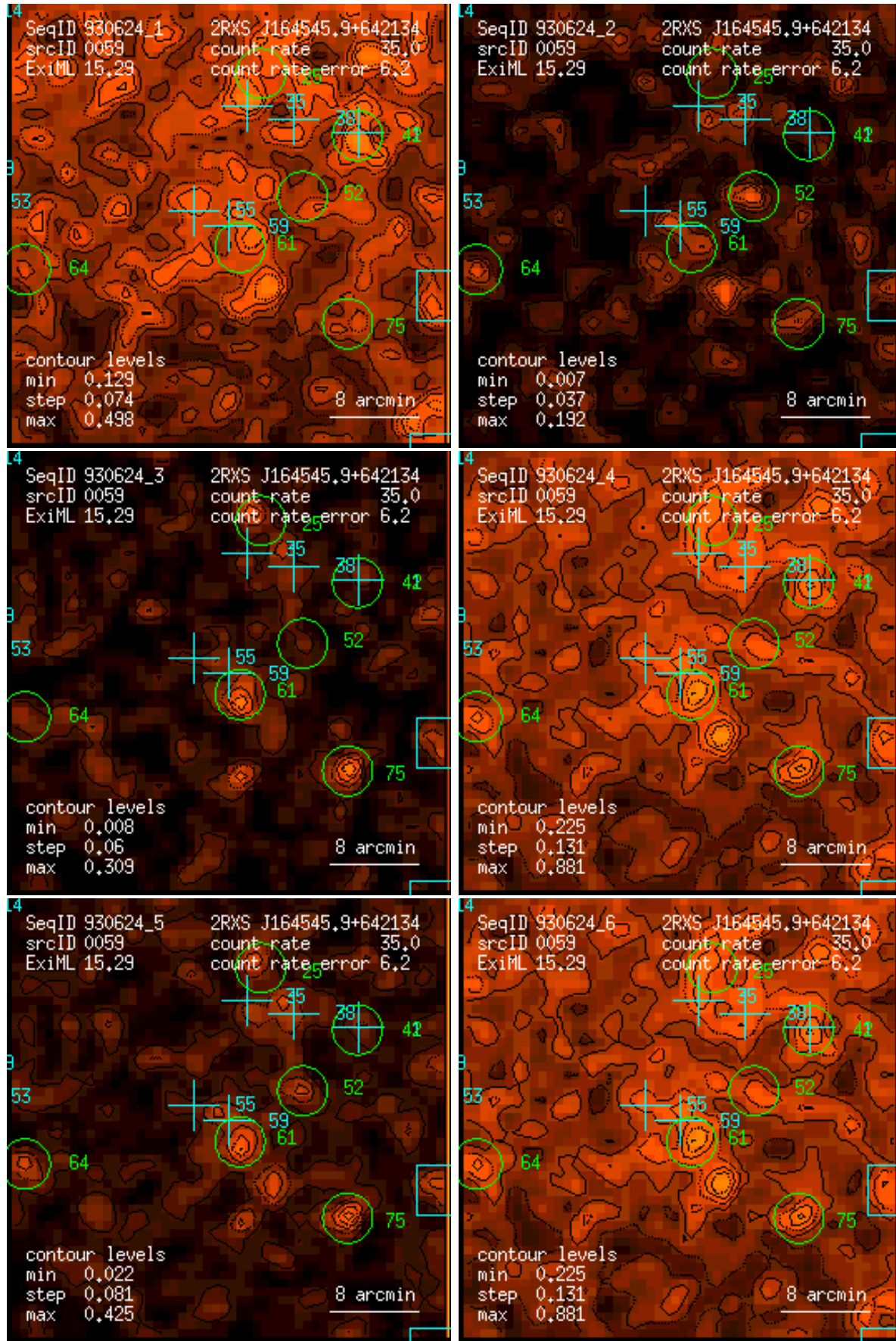
Figure 59: RASS 930624: detection 0059: band rate images, Gaussian filter: (1) PSPC channels 11 – 41, (2) 52 – 90, (3) 91 – 201, (4) 11 – 235, (5) 52 – 201, (6) 11 – 201. Broad band rates in counts/ks. Band rate contour levels in counts/ks/arcmin 2 .
