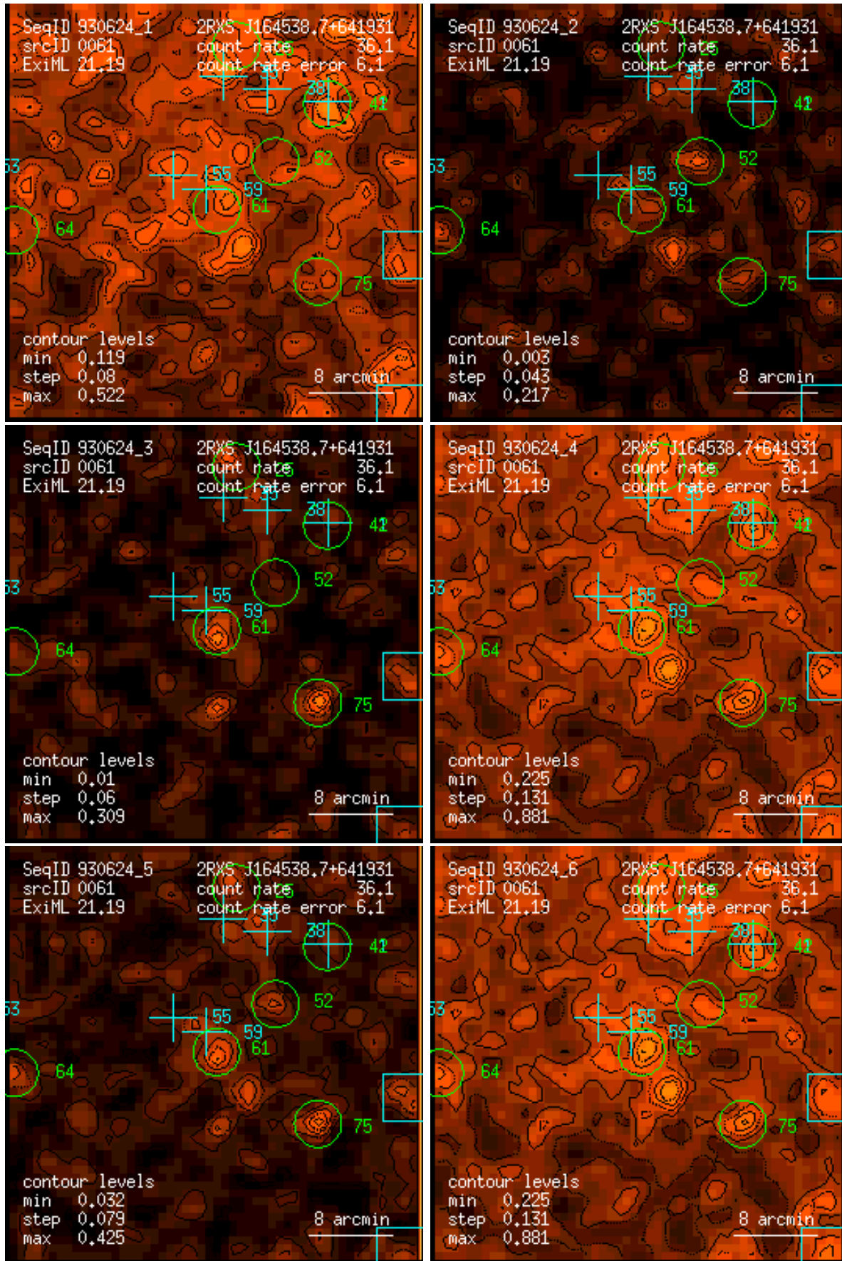
Figure 61: RASS 930624: detection 0061: band rate images, Gaussian filter: (1) PSPC channels 11 – 41, (2) 52 – 90, (3) 91 – 201, (4) 11 – 235, (5) 52 – 201, (6) 11 – 201. Broad band rates in counts/ks. Band rate contour levels in counts/ks/arcmin 2 .
