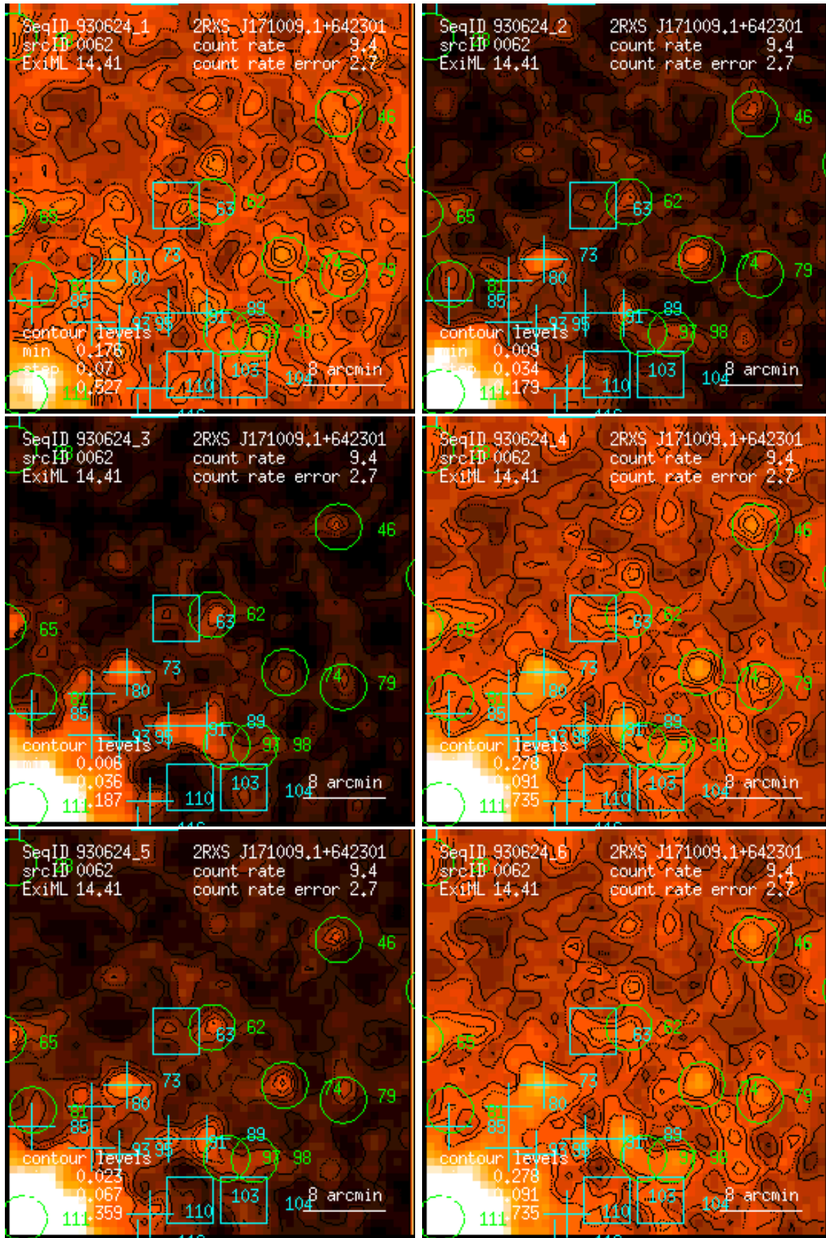
Figure 62: RASS 930624: detection 0062: band rate images, Gaussian filter: (1) PSPC channels 11 – 41, (2) 52 – 90, (3) 91 – 201, (4) 11 – 235, (5) 52 – 201, (6) 11 – 201. Broad band rates in counts/ks. Band rate contour levels in counts/ks/arcmin 2 .
