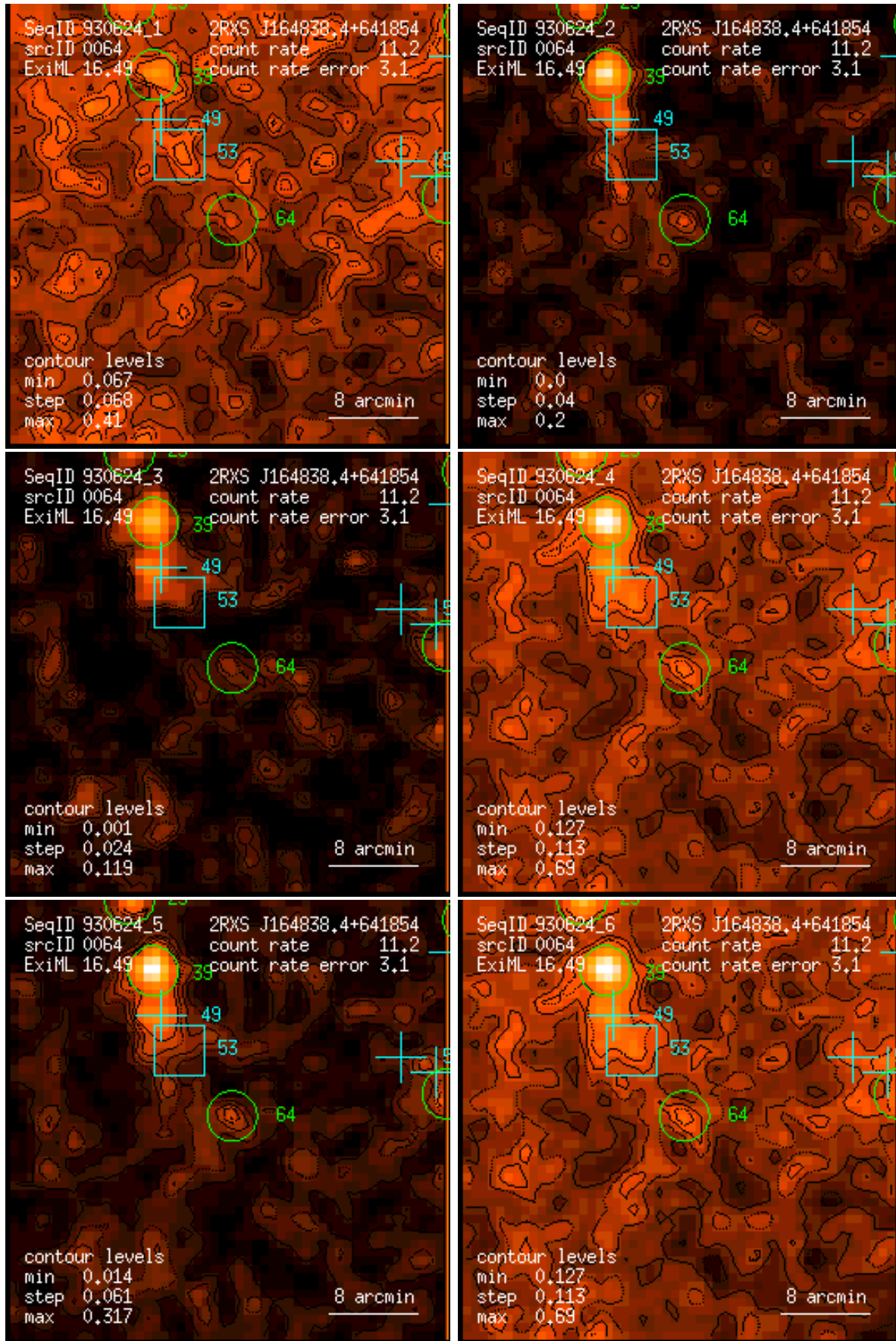
Figure 64: RASS 930624: detection 0064: band rate images, Gaussian filter: (1) PSPC channels 11 – 41, (2) 52 – 90, (3) 91 – 201, (4) 11 – 235, (5) 52 – 201, (6) 11 – 201. Broad band rates in counts/ks. Band rate contour levels in counts/ks/arcmin 2 .
