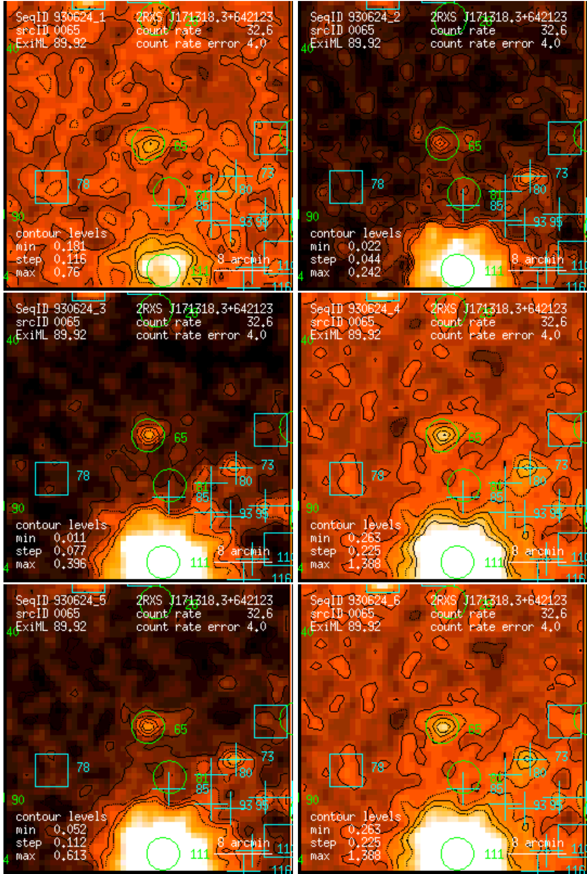
Figure 65: RASS 930624: detection 0065: band rate images, Gaussian filter: (1) PSPC channels 11 – 41, (2) 52 – 90, (3) 91 – 201, (4) 11 – 235, (5) 52 – 201, (6) 11 – 201. Broad band rates in counts/ks. Band rate contour levels in counts/ks/arcmin 2 .
