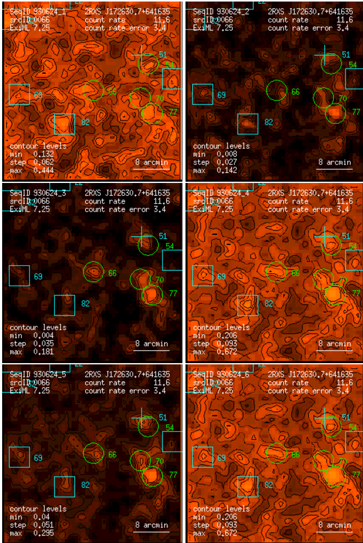
Figure 66: RASS 930624: detection 0066: band rate images, Gaussian filter: (1) PSPC channels 11 – 41, (2) 52 – 90, (3) 91 – 201, (4) 11 – 235, (5) 52 – 201, (6) 11 – 201. Broad band rates in counts/ks. Band rate contour levels in counts/ks/arcmin 2 .
