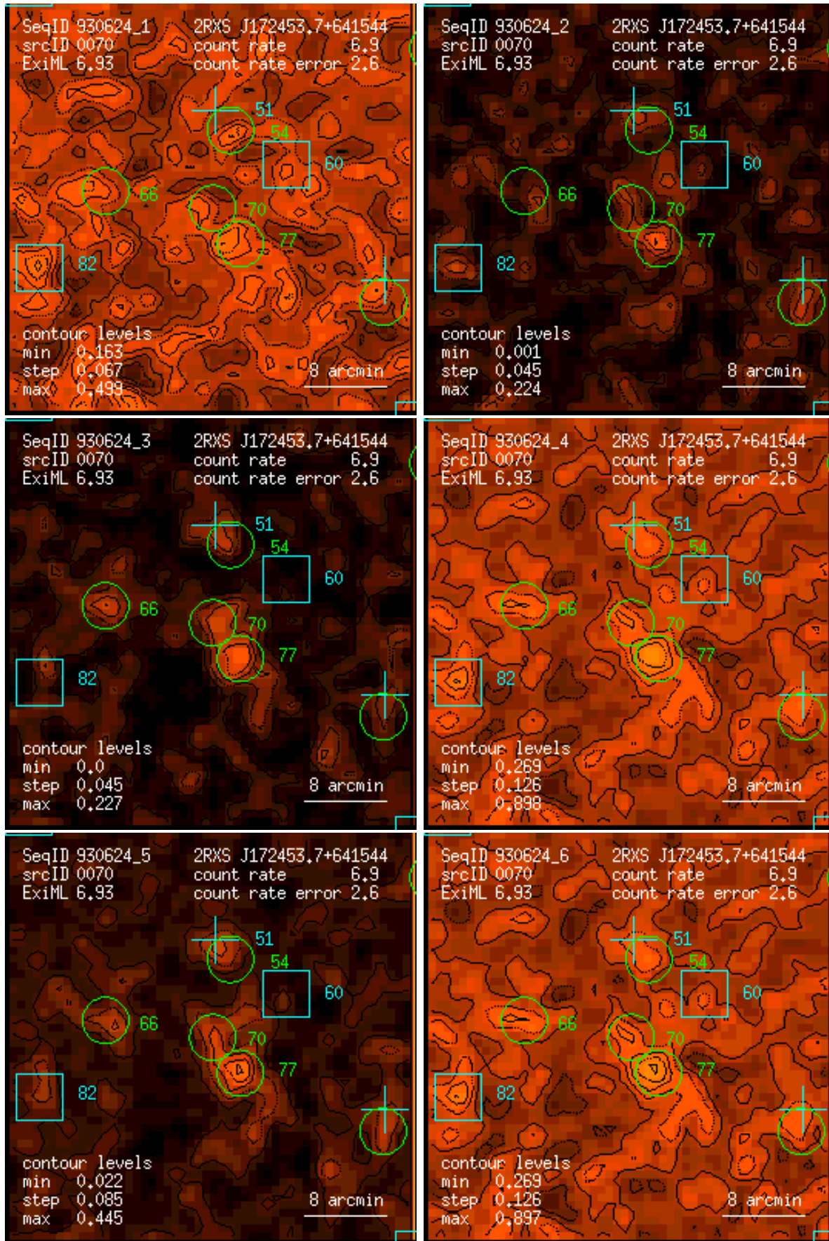
Figure 70: RASS 930624: detection 0070: band rate images, Gaussian filter: (1) PSPC channels 11 – 41, (2) 52 – 90, (3) 91 – 201, (4) 11 – 235, (5) 52 – 201, (6) 11 – 201. Broad band rates in counts/ks. Band rate contour levels in counts/ks/arcmin 2 .
