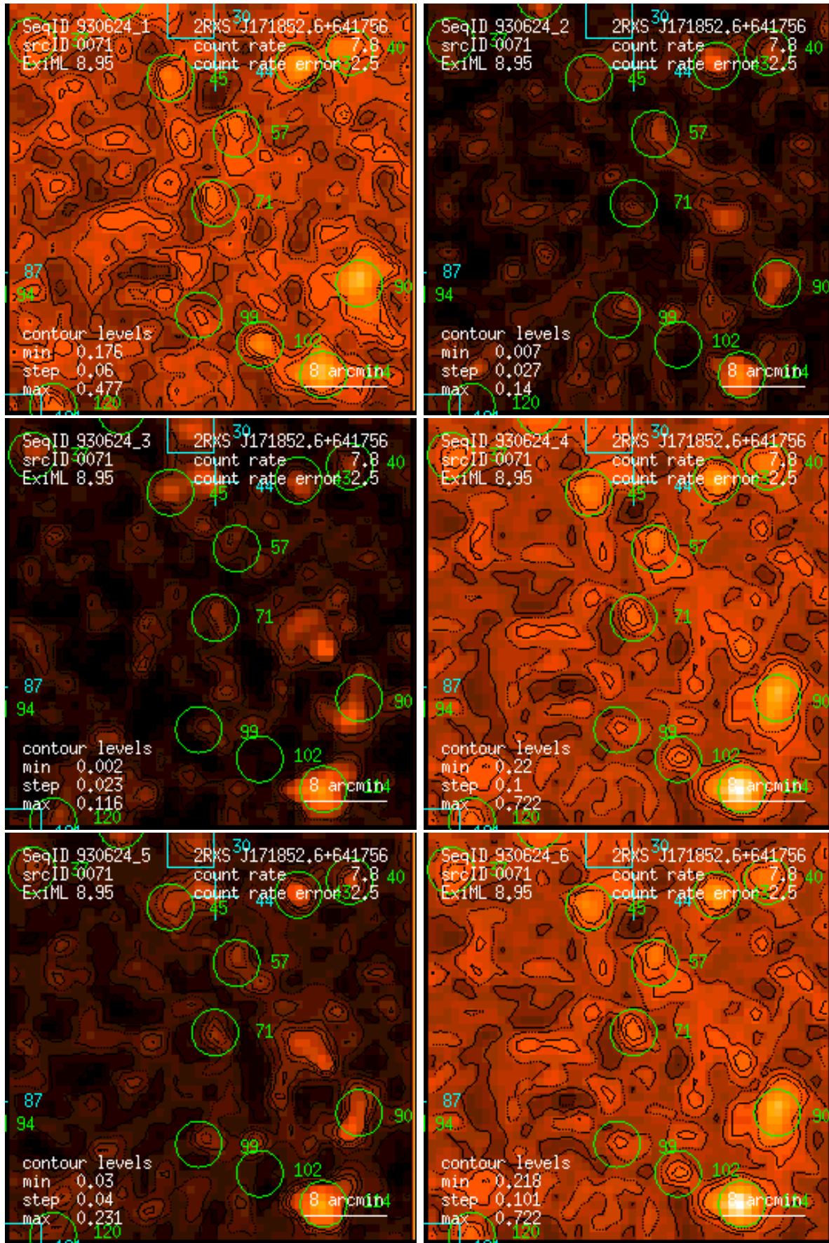
Figure 71: RASS 930624: detection 0071: band rate images, Gaussian filter: (1) PSPC channels 11 – 41, (2) 52 – 90, (3) 91 – 201, (4) 11 – 235, (5) 52 – 201, (6) 11 – 201. Broad band rates in counts/ks. Band rate contour levels in counts/ks/arcmin 2 .
