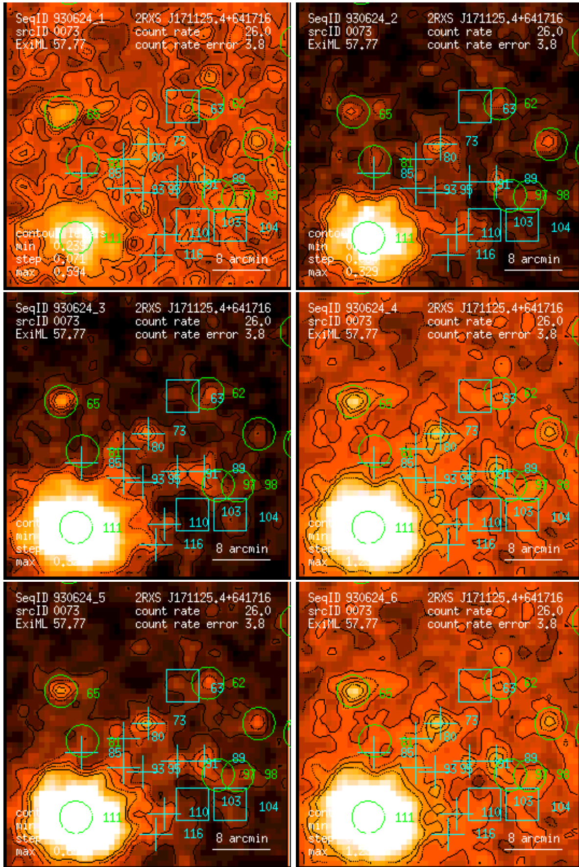
Figure 73: RASS 930624: detection 0073: band rate images, Gaussian filter: (1) PSPC channels 11 – 41, (2) 52 – 90, (3) 91 – 201, (4) 11 – 235, (5) 52 – 201, (6) 11 – 201. Broad band rates in counts/ks. Band rate contour levels in counts/ks/arcmin 2 .
