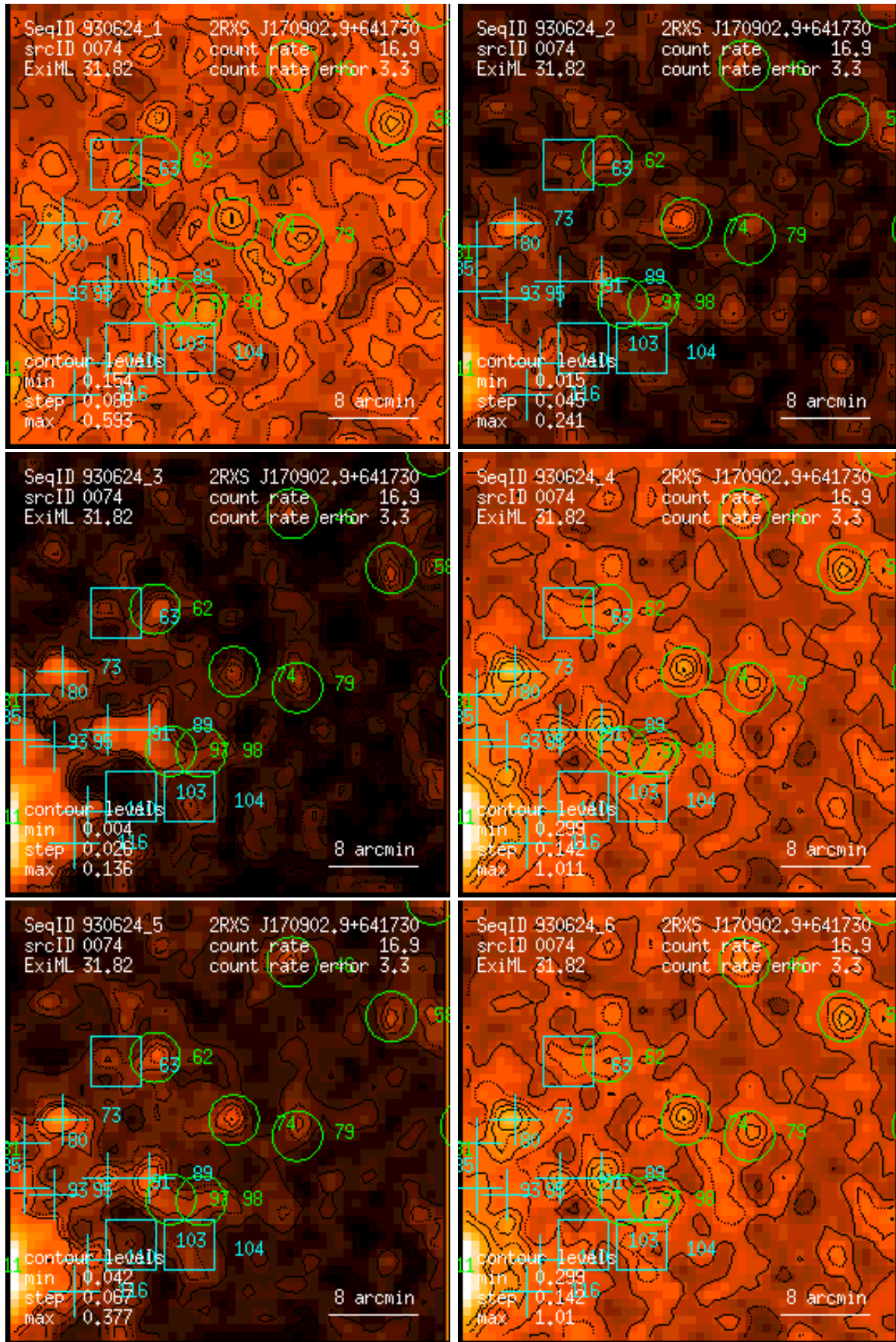
Figure 74: RASS 930624: detection 0074: band rate images, Gaussian filter: (1) PSPC channels 11 – 41, (2) 52 – 90, (3) 91 – 201, (4) 11 – 235, (5) 52 – 201, (6) 11 – 201. Broad band rates in counts/ks. Band rate contour levels in counts/ks/arcmin 2 .
