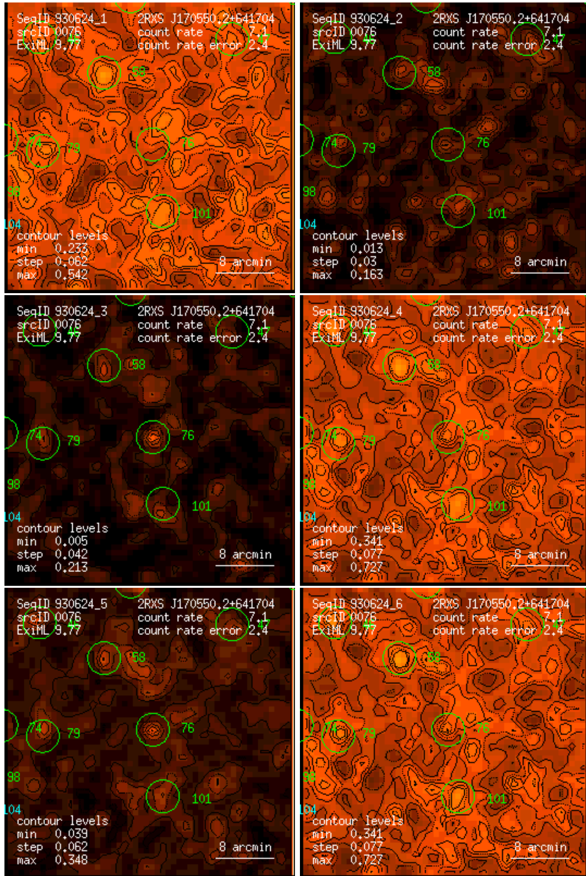
Figure 76: RASS 930624: detection 0076: band rate images, Gaussian filter: (1) PSPC channels 11 – 41, (2) 52 – 90, (3) 91 – 201, (4) 11 – 235, (5) 52 – 201, (6) 11 – 201. Broad band rates in counts/ks. Band rate contour levels in counts/ks/arcmin 2 .
