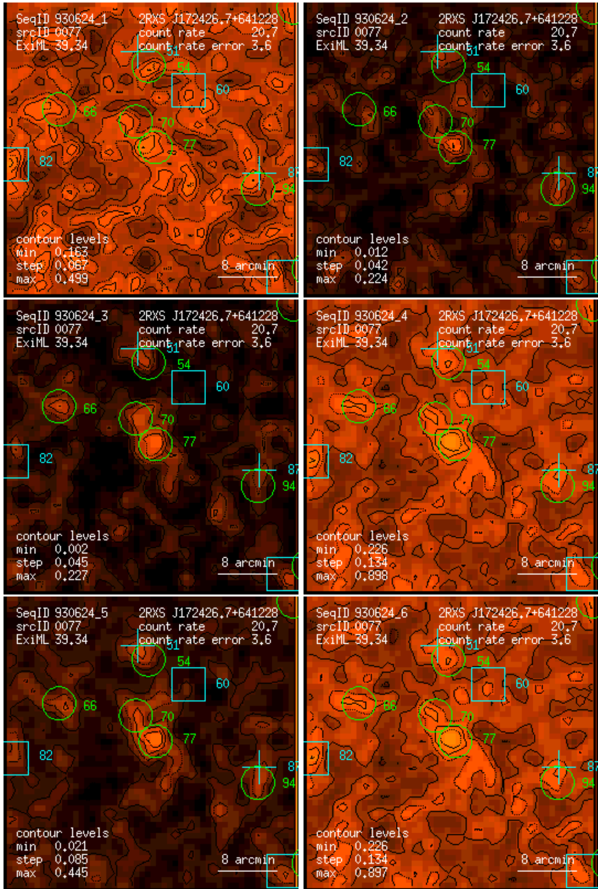
Figure 77: RASS 930624: detection 0077: band rate images, Gaussian filter: (1) PSPC channels 11 – 41, (2) 52 – 90, (3) 91 – 201, (4) 11 – 235, (5) 52 – 201, (6) 11 – 201. Broad band rates in counts/ks. Band rate contour levels in counts/ks/arcmin 2 .
