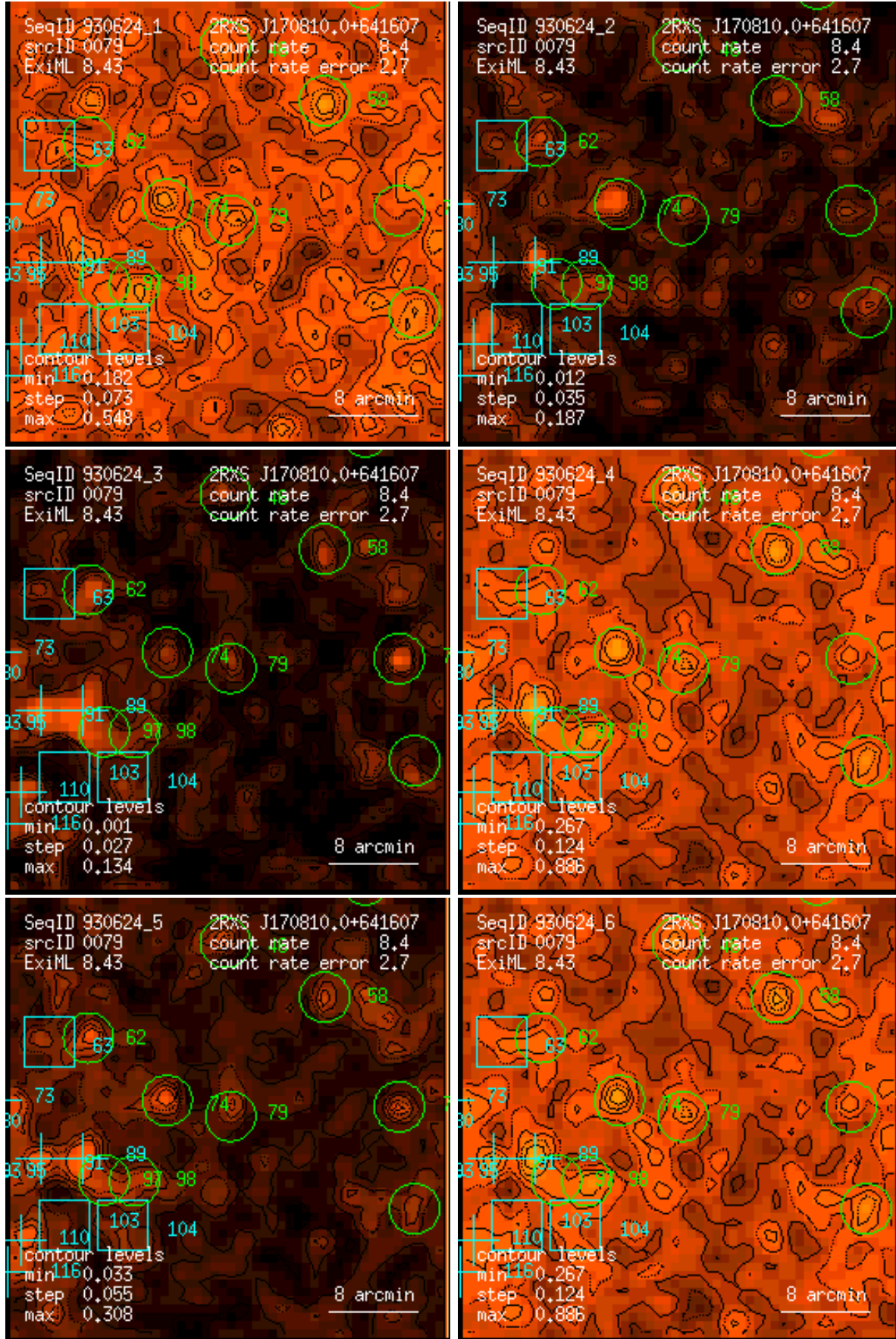
Figure 79: RASS 930624: detection 0079: band rate images, Gaussian filter: (1) PSPC channels 11 – 41, (2) 52 – 90, (3) 91 – 201, (4) 11 – 235, (5) 52 – 201, (6) 11 – 201. Broad band rates in counts/ks. Band rate contour levels in counts/ks/arcmin 2 .
