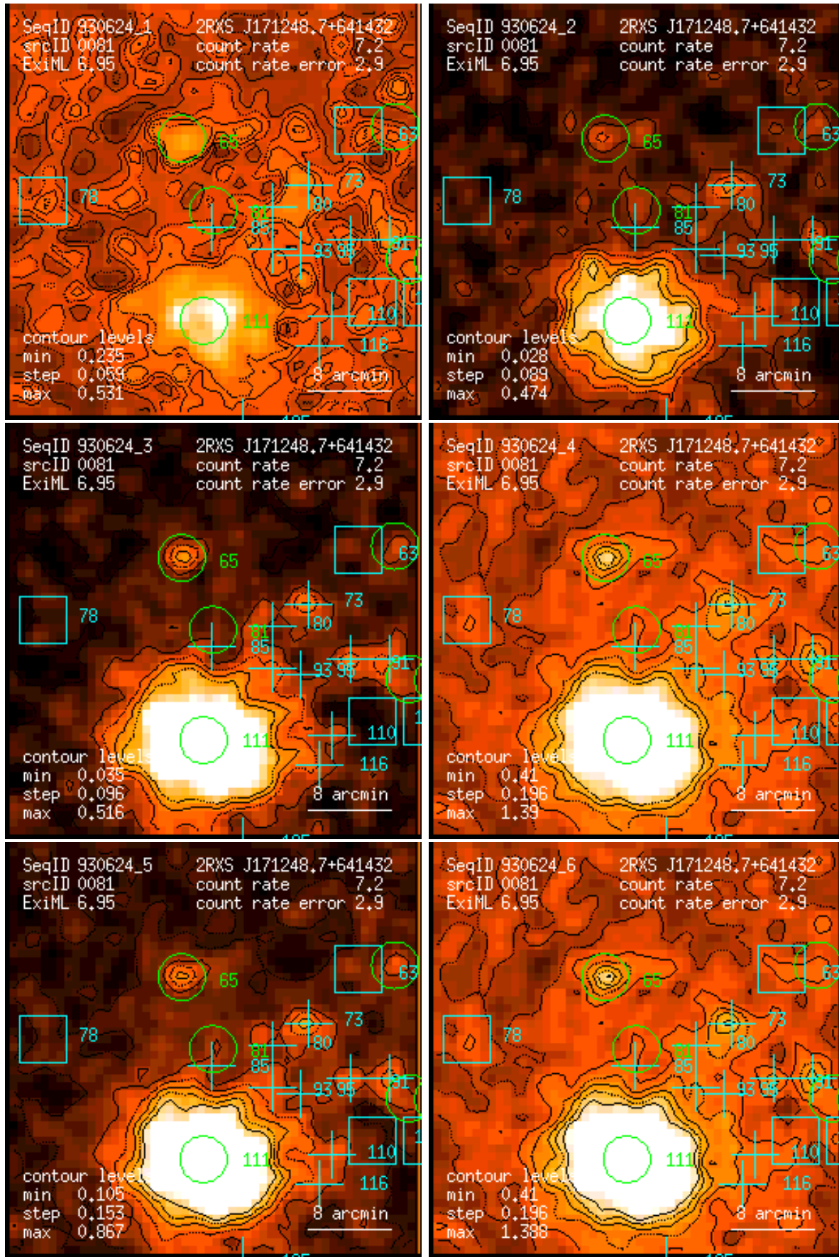
Figure 81: RASS 930624: detection 0081: band rate images, Gaussian filter: (1) PSPC channels 11 – 41, (2) 52 – 90, (3) 91 – 201, (4) 11 – 235, (5) 52 – 201, (6) 11 – 201. Broad band rates in counts/ks. Band rate contour levels in counts/ks/arcmin 2 .
