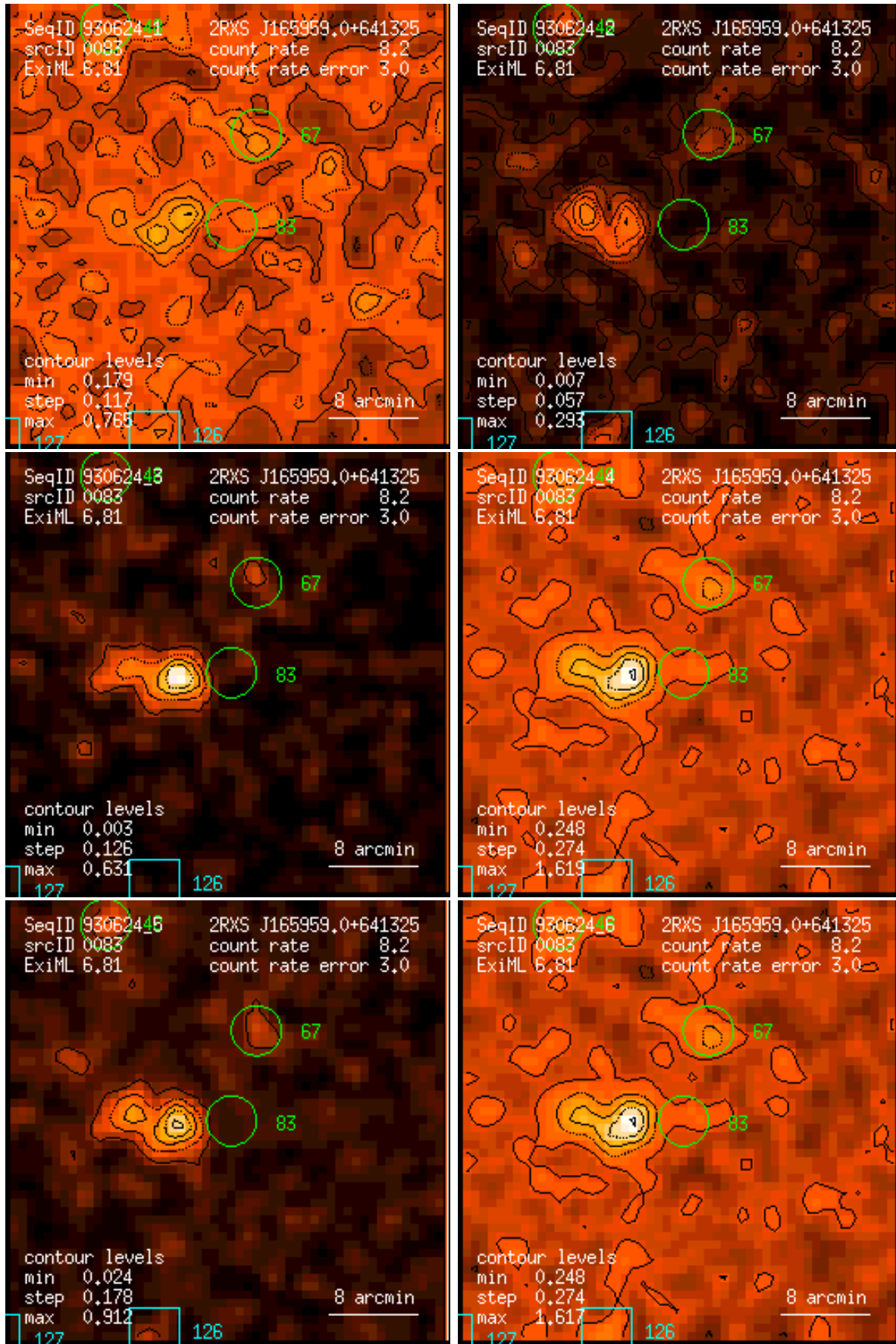
Figure 83: RASS 930624: detection 0083: band rate images, Gaussian filter: (1) PSPC channels 11 – 41, (2) 52 – 90, (3) 91 – 201, (4) 11 – 235, (5) 52 – 201, (6) 11 – 201. Broad band rates in counts/ks. Band rate contour levels in counts/ks/arcmin 2 .
