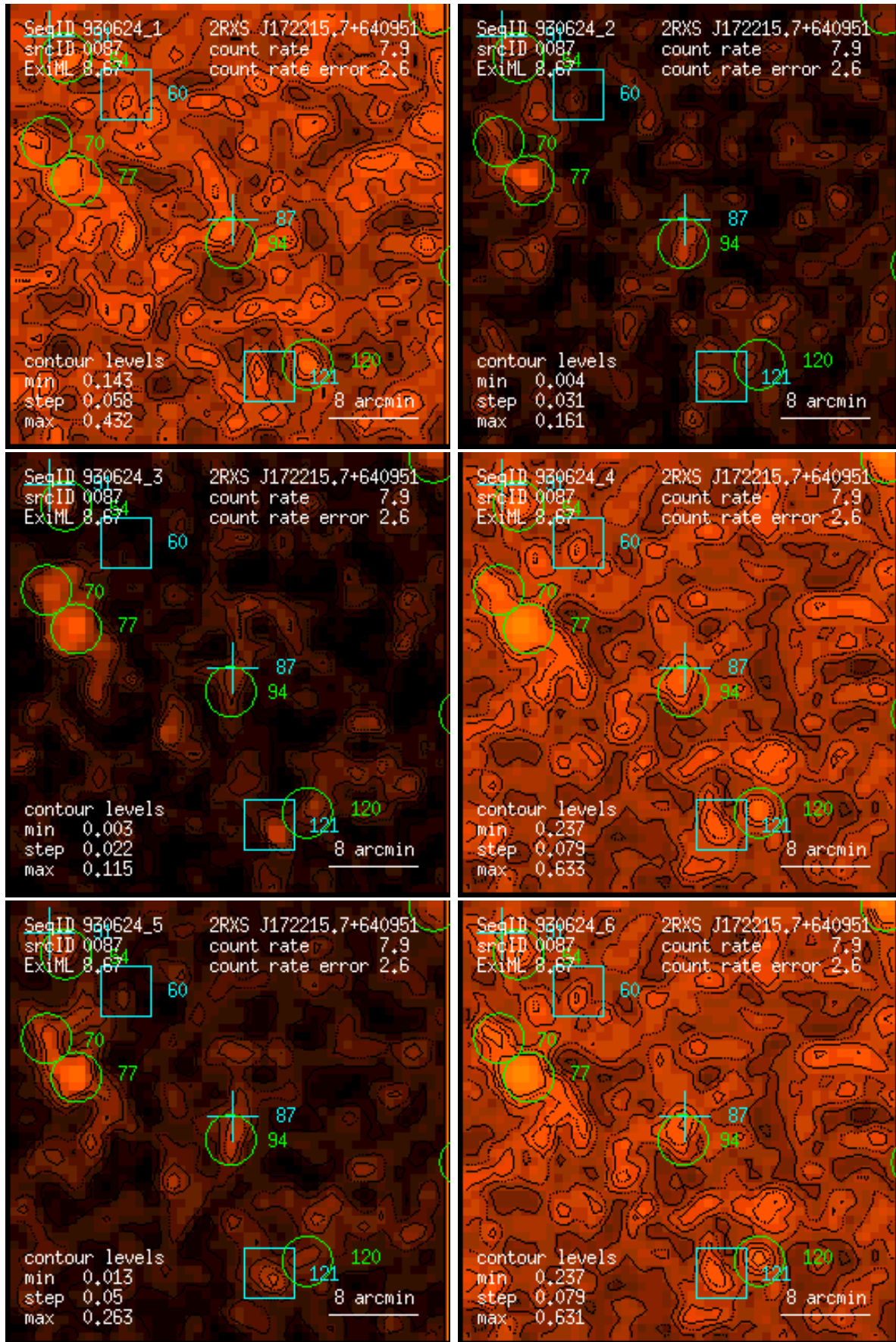
Figure 87: RASS 930624: detection 0087: band rate images, Gaussian filter: (1) PSPC channels 11 – 41, (2) 52 – 90, (3) 91 – 201, (4) 11 – 235, (5) 52 – 201, (6) 11 – 201. Broad band rates in counts/ks. Band rate contour levels in counts/ks/arcmin 2 .
