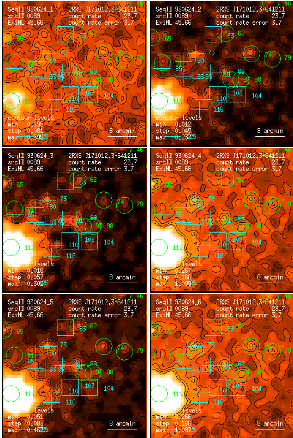
Figure 89: RASS 930624: detection 0089: band rate images, Gaussian filter: (1) PSPC channels 11 – 41, (2) 52 – 90, (3) 91 – 201, (4) 11 – 235, (5) 52 – 201, (6) 11 – 201. Broad band rates in counts/ks. Band rate contour levels in counts/ks/arcmin 2 .
