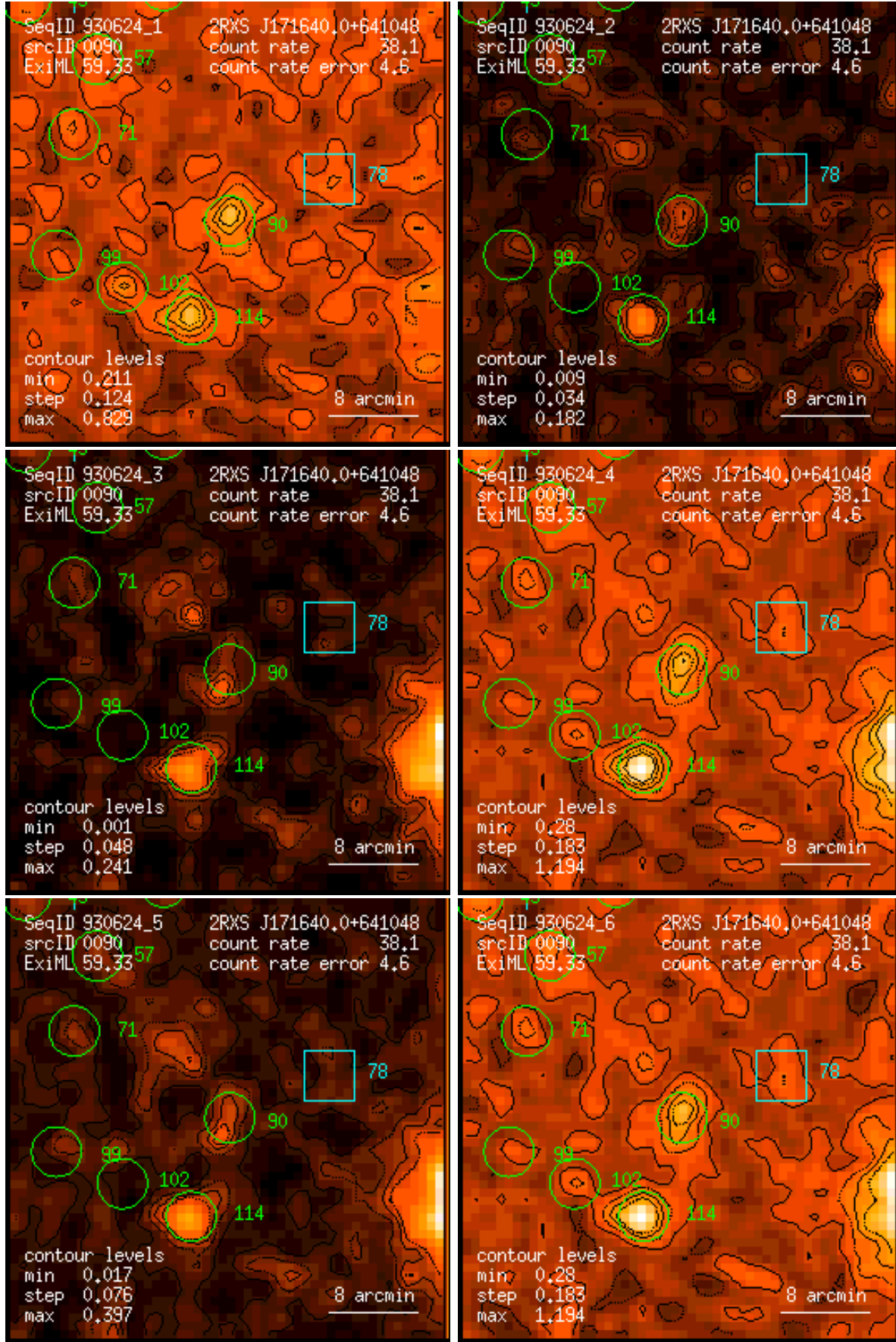
Figure 90: RASS 930624: detection 0090: band rate images, Gaussian filter: (1) PSPC channels 11 – 41, (2) 52 – 90, (3) 91 – 201, (4) 11 – 235, (5) 52 – 201, (6) 11 – 201. Broad band rates in counts/ks. Band rate contour levels in counts/ks/arcmin 2 .
