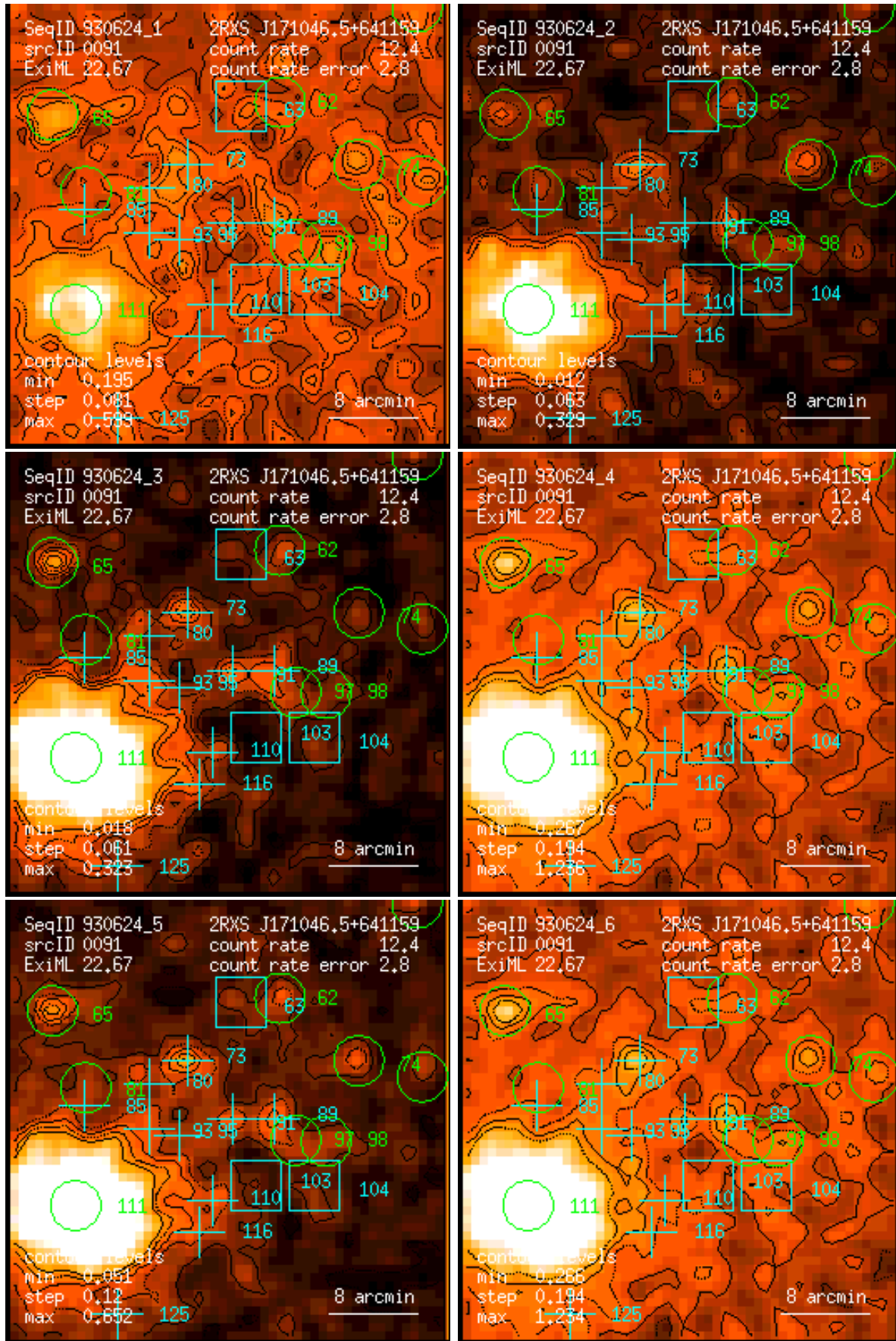
Figure 91: RASS 930624: detection 0091: band rate images, Gaussian filter: (1) PSPC channels 11 – 41, (2) 52 – 90, (3) 91 – 201, (4) 11 – 235, (5) 52 – 201, (6) 11 – 201. Broad band rates in counts/ks. Band rate contour levels in counts/ks/arcmin 2 .
